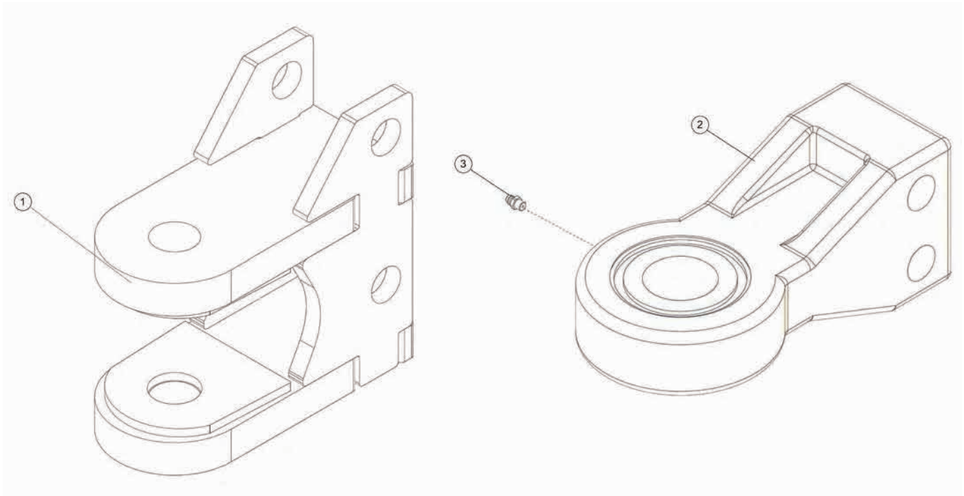
FIGURE 25 OPTIONAL PSOCH - CLEVIS HITCH OPTIONAL HTCHB - BULLNOSE HITCH
