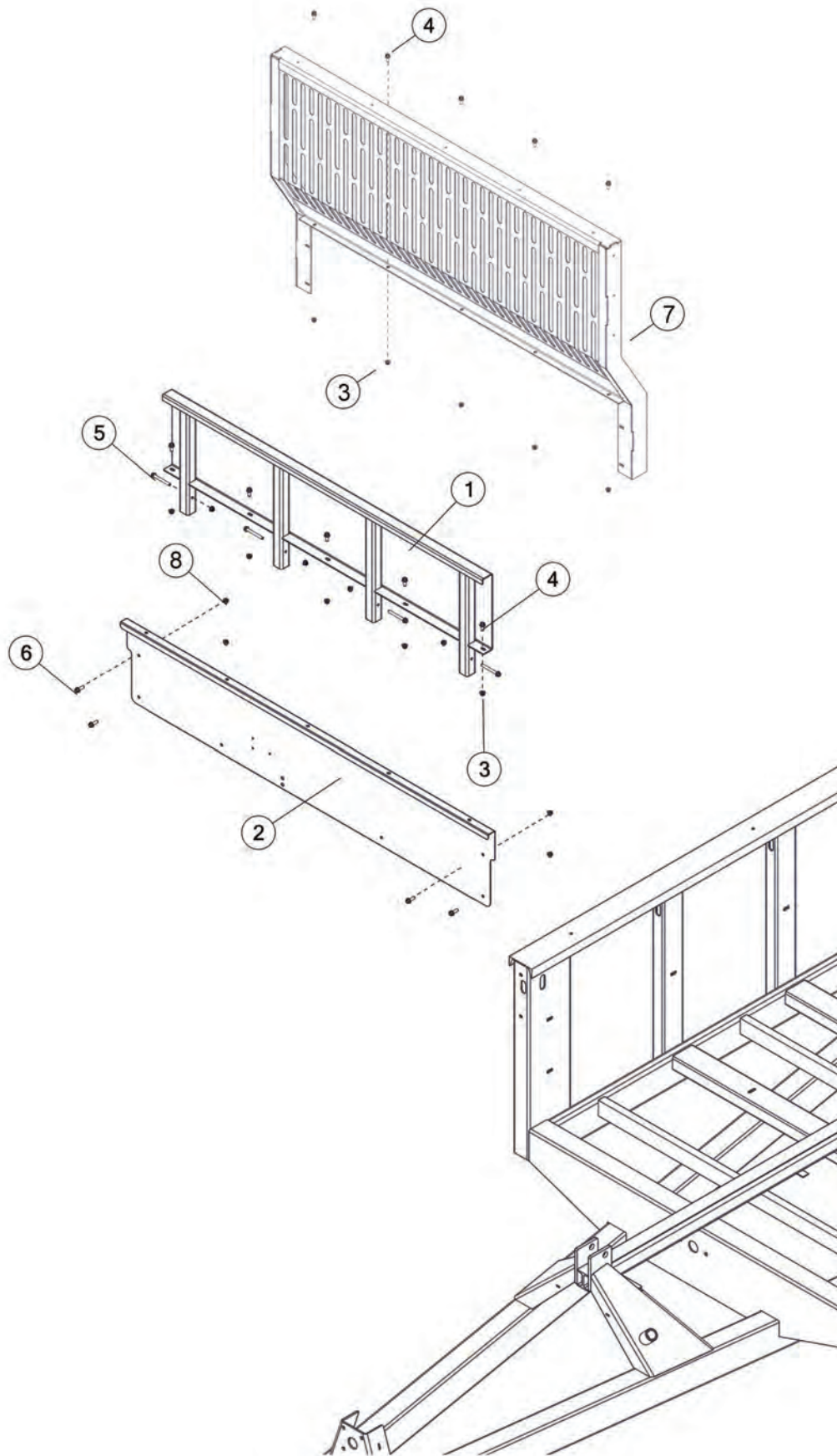
FIGURE 5 PUSHER EXTENSION & COMPONENTS
