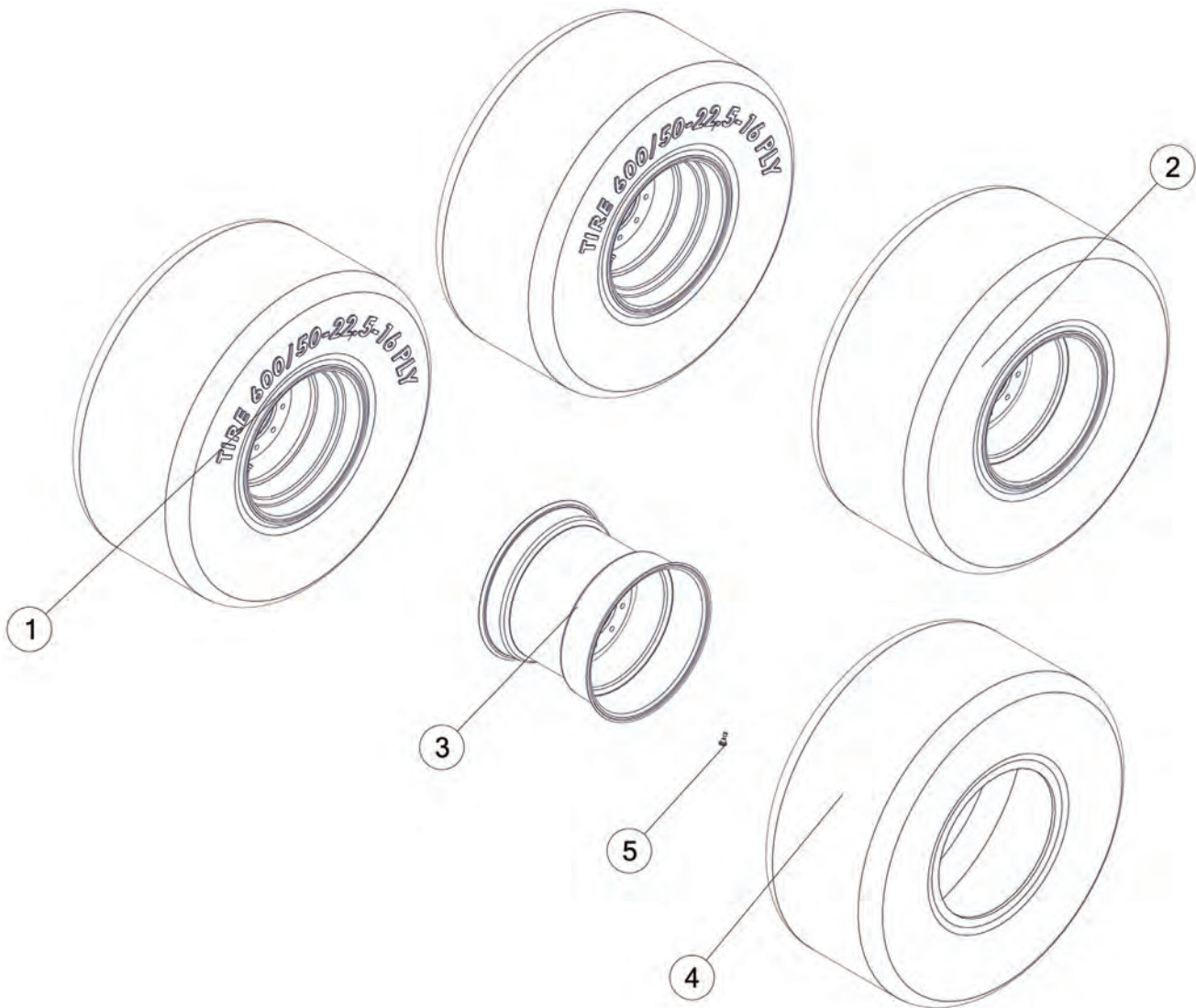
FIGURE 3 OPTIONAL TWP600S TIRE & WHEEL PACKAGE
