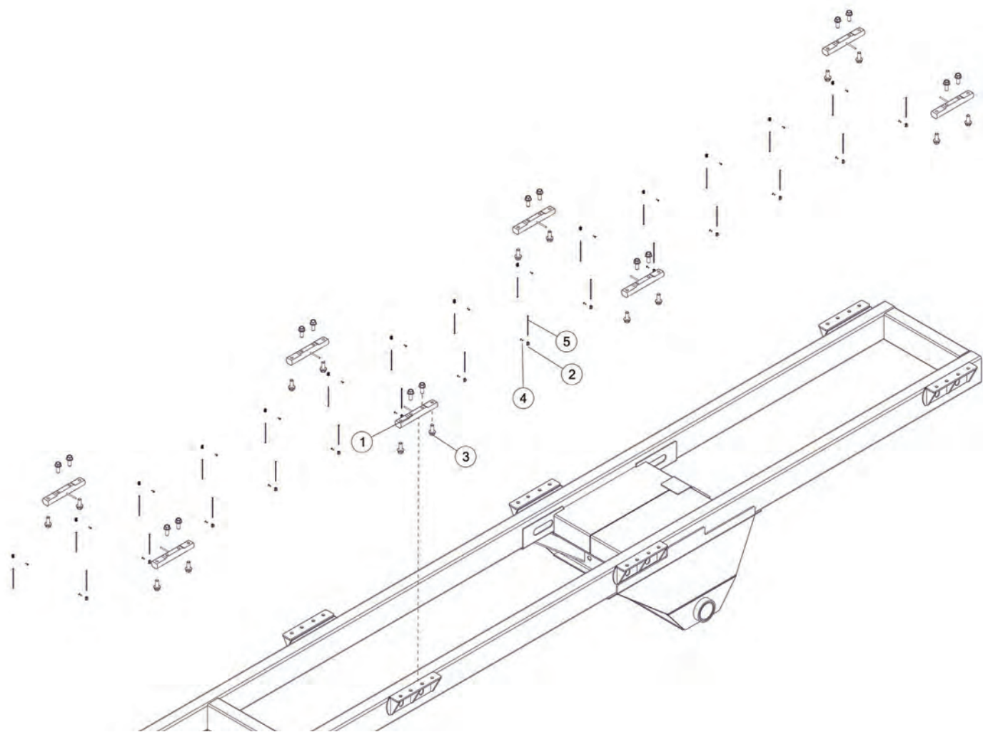
FIGURE 6 OPTIONAL CHO8SCL SCALE SYSTEM
