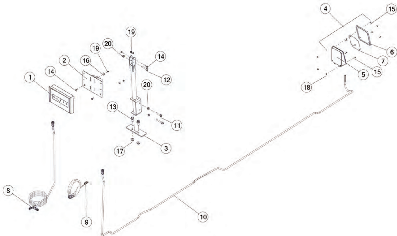
FIGURE 6 OPTIONAL CHO8SCL SCALE SYSTEM
