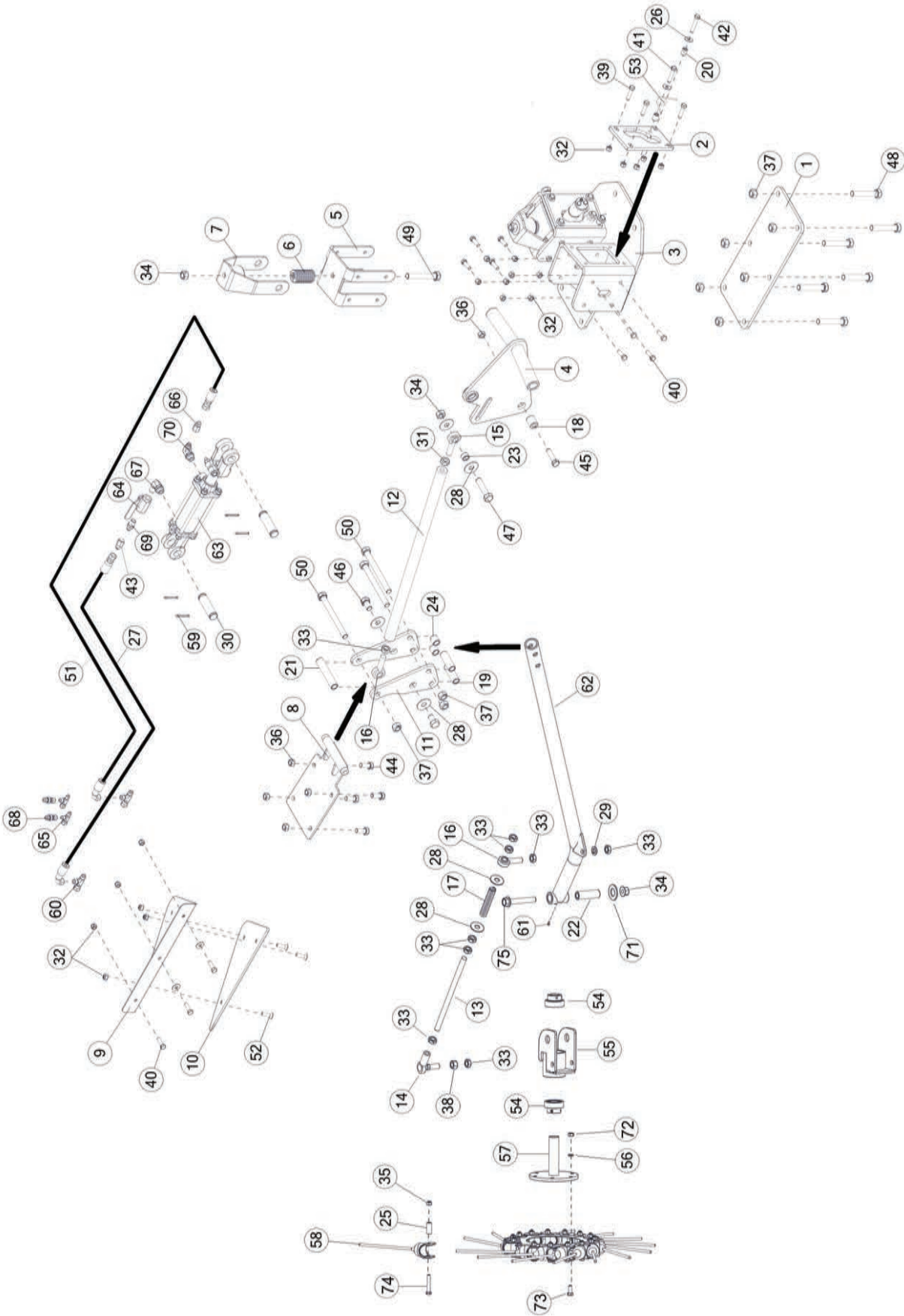
FIGURE 17 OPTIONAL KICKER WHEEL
