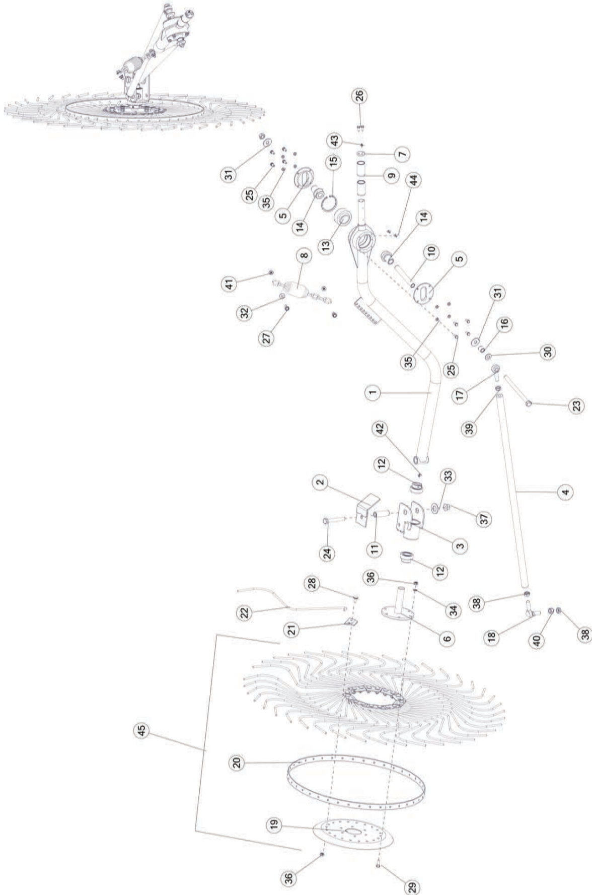
FIGURE 17 OPTIONAL KICKER WHEEL
