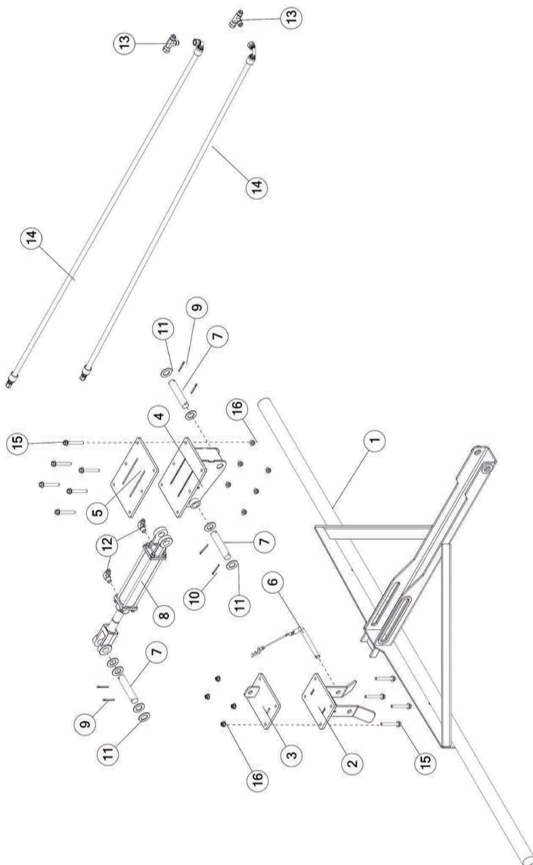
FIGURE 16 OPTIONAL CORN STALK BREAKER
