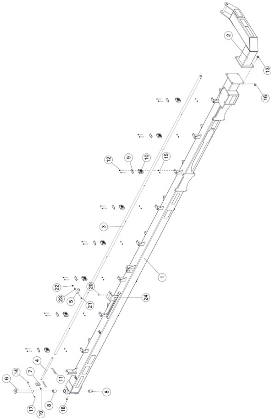
FIGURE 7 MAIN RAKE BEAM ARM RH & COMPONENTS
