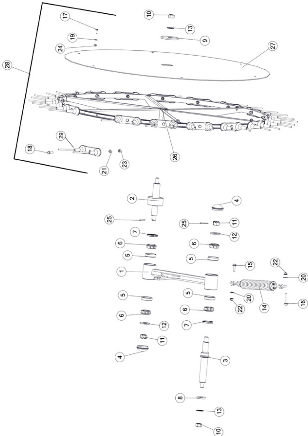
FIGURE 10 RAKE WHEEL & COMPONENTS
