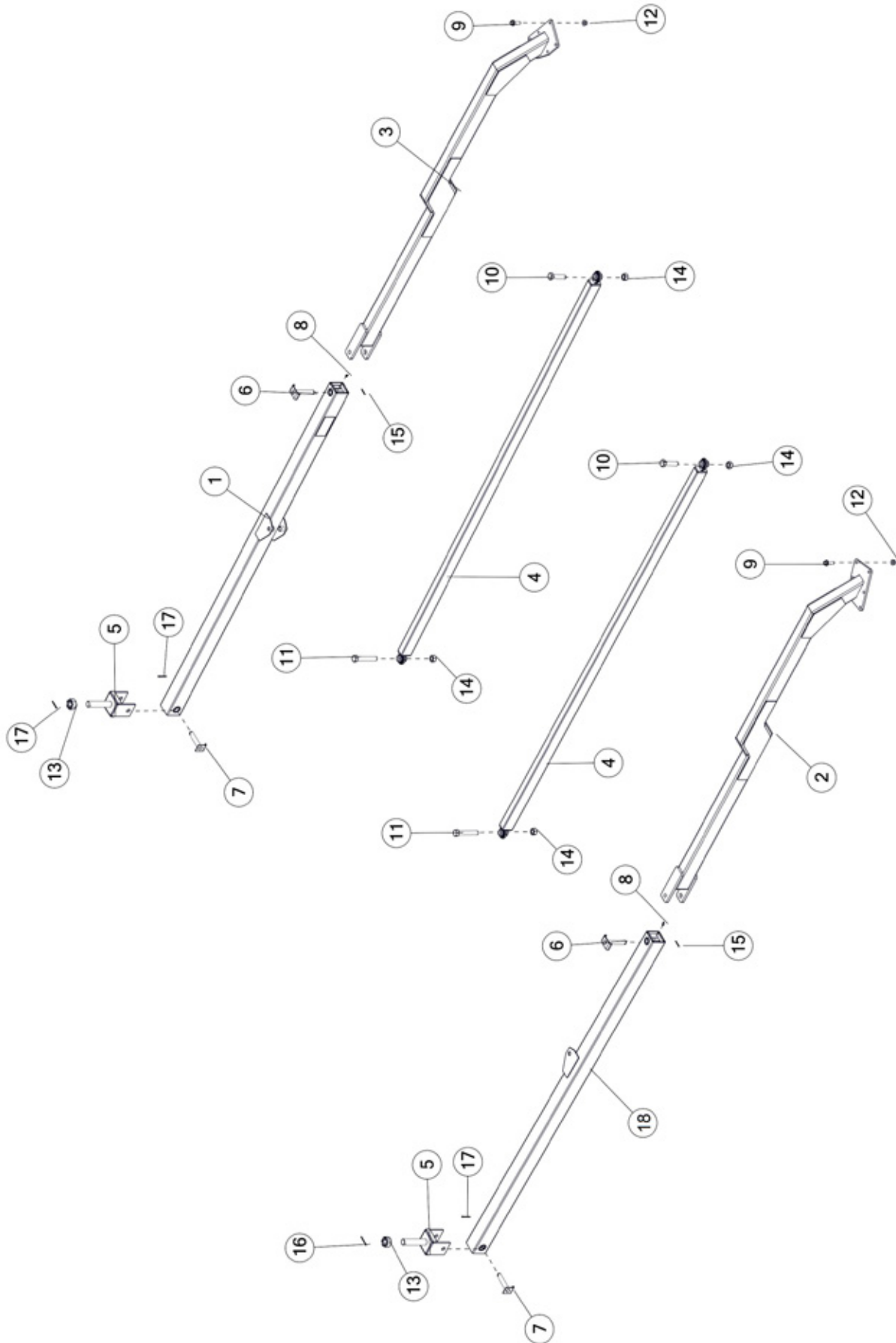
FIGURE 6 LINKAGE ARMS & COMPONENTS
