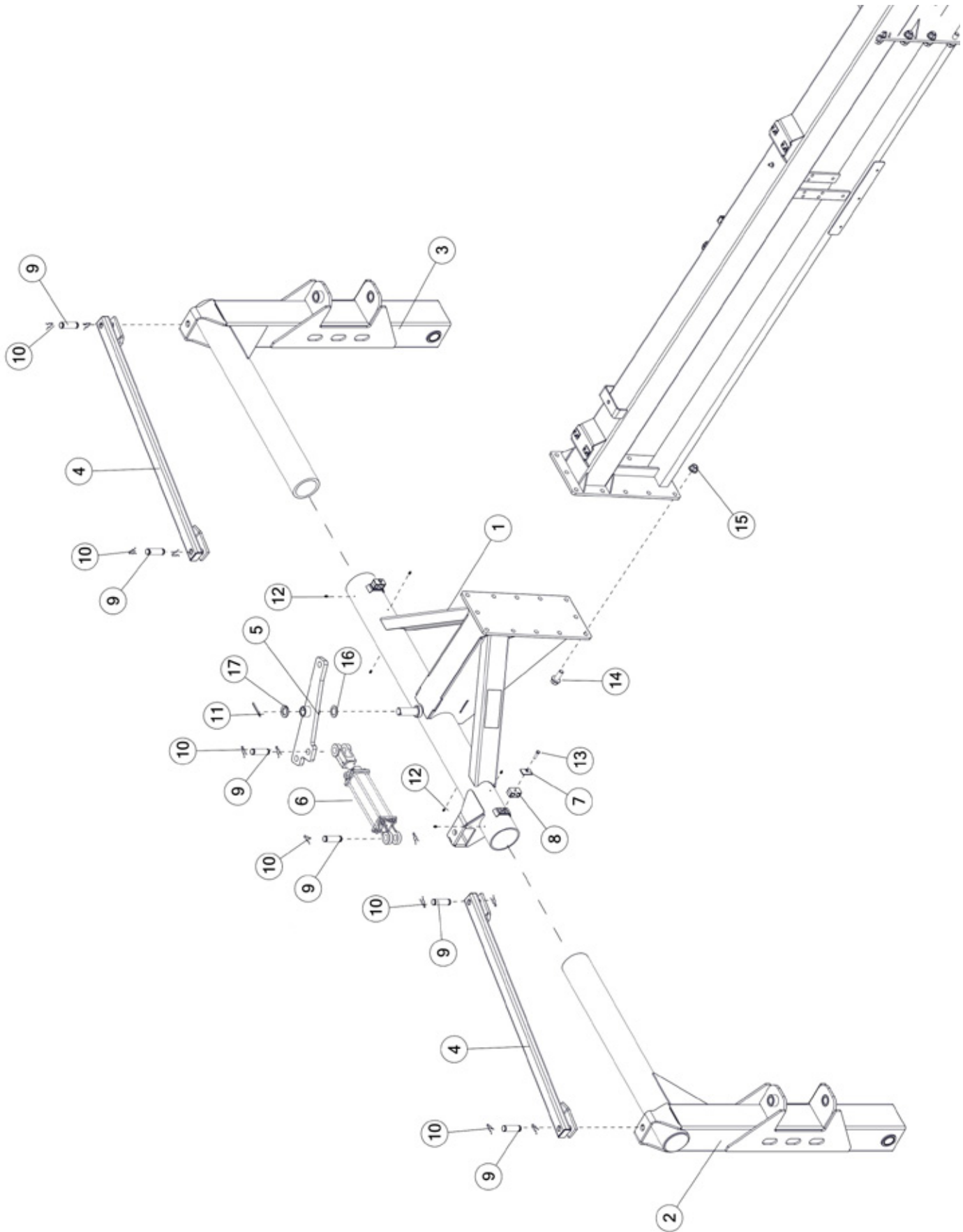
FIGURE 4 MAIN FRAME REAR & UPRIGHTS
