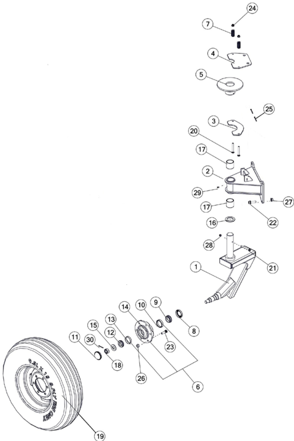
FIGURE 9 FRONT CASTER & COMPONENTS
