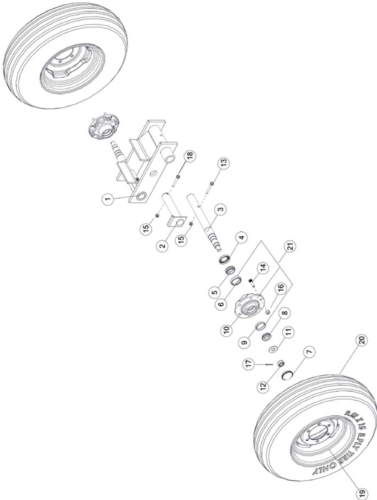
FIGURE 5 TANDEMS & TIRES
