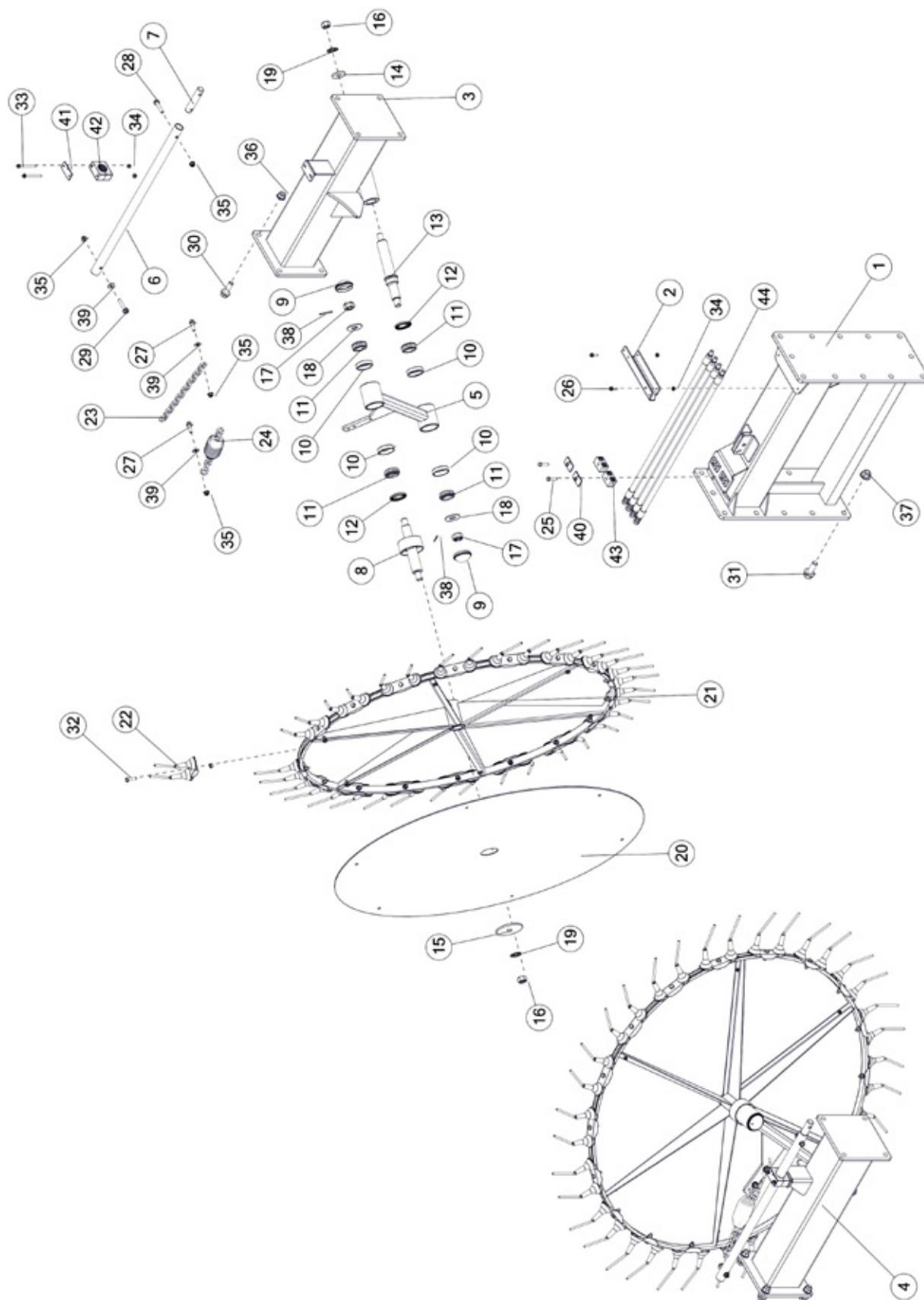
FIGURE 15 2 WHEEL EXTENSION OPTION
