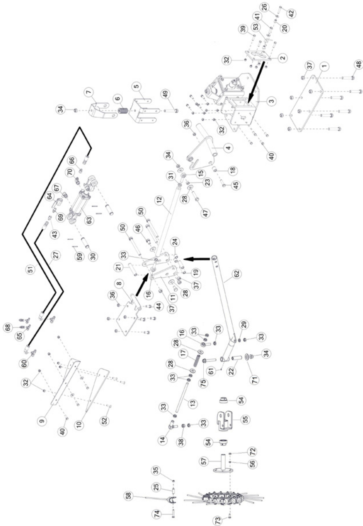
FIGURE 18 OPTIONAL KICKER WHEEL
