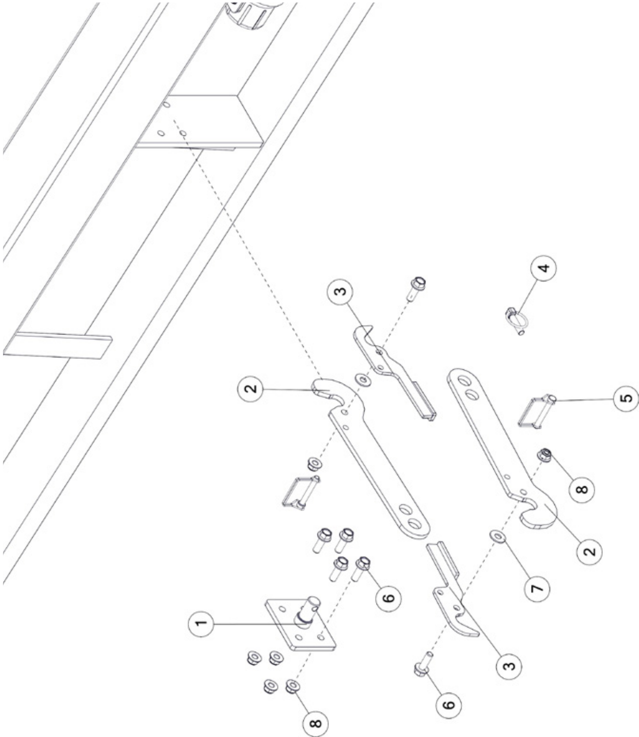
FIGURE 2 TRANSPORT LOCK & COMPONENTS
