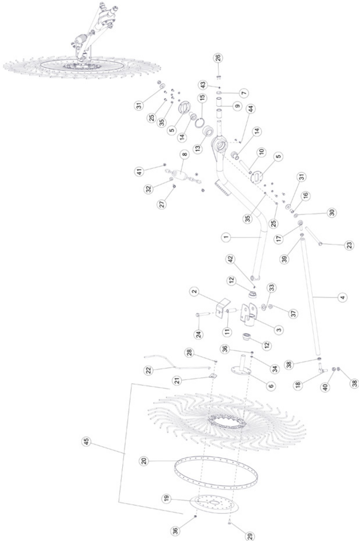
FIGURE 18 OPTIONAL KICKER WHEEL
