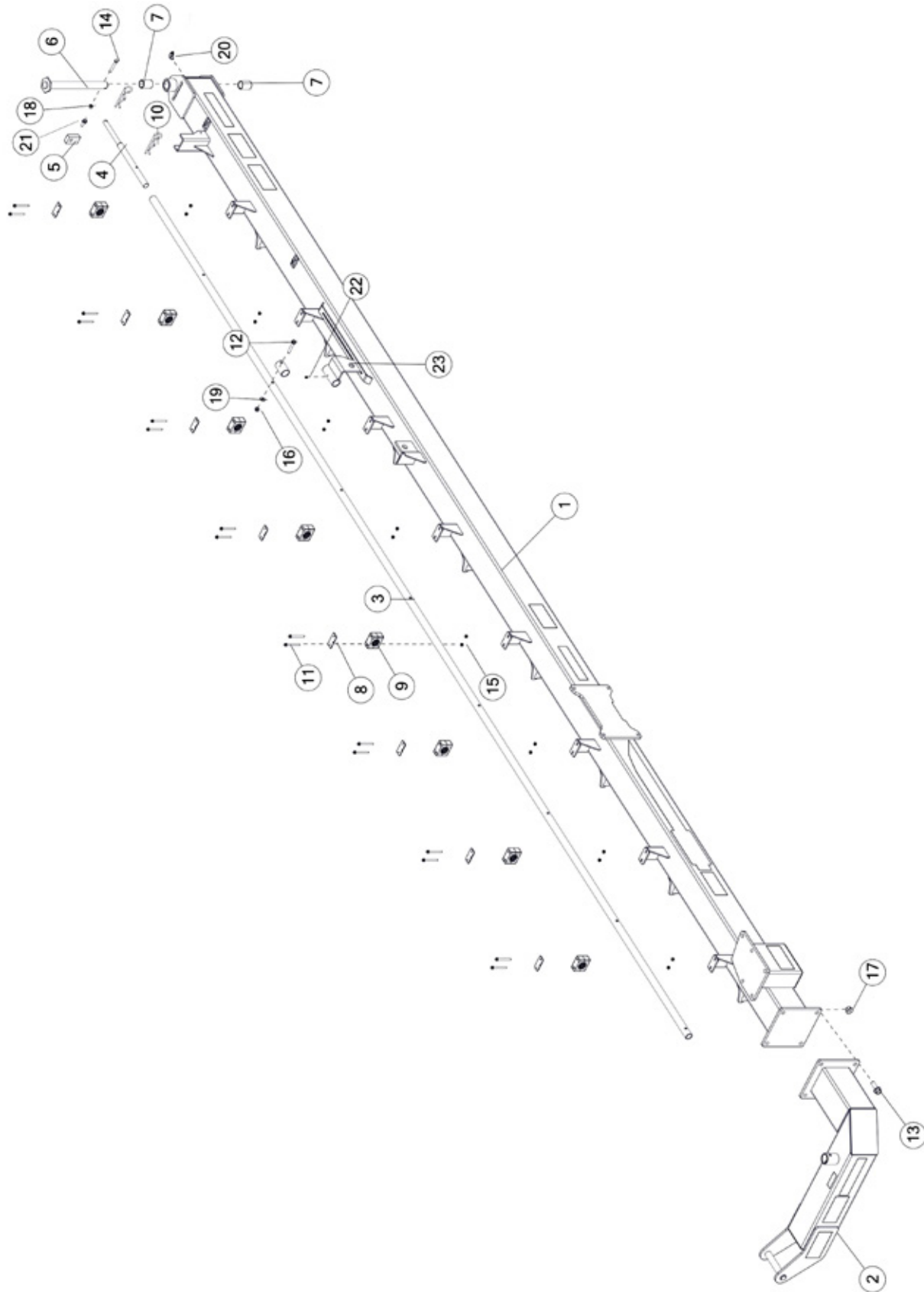
FIGURE 8 MAIN RAKE BEAM ARM LH & COMPONENTS
