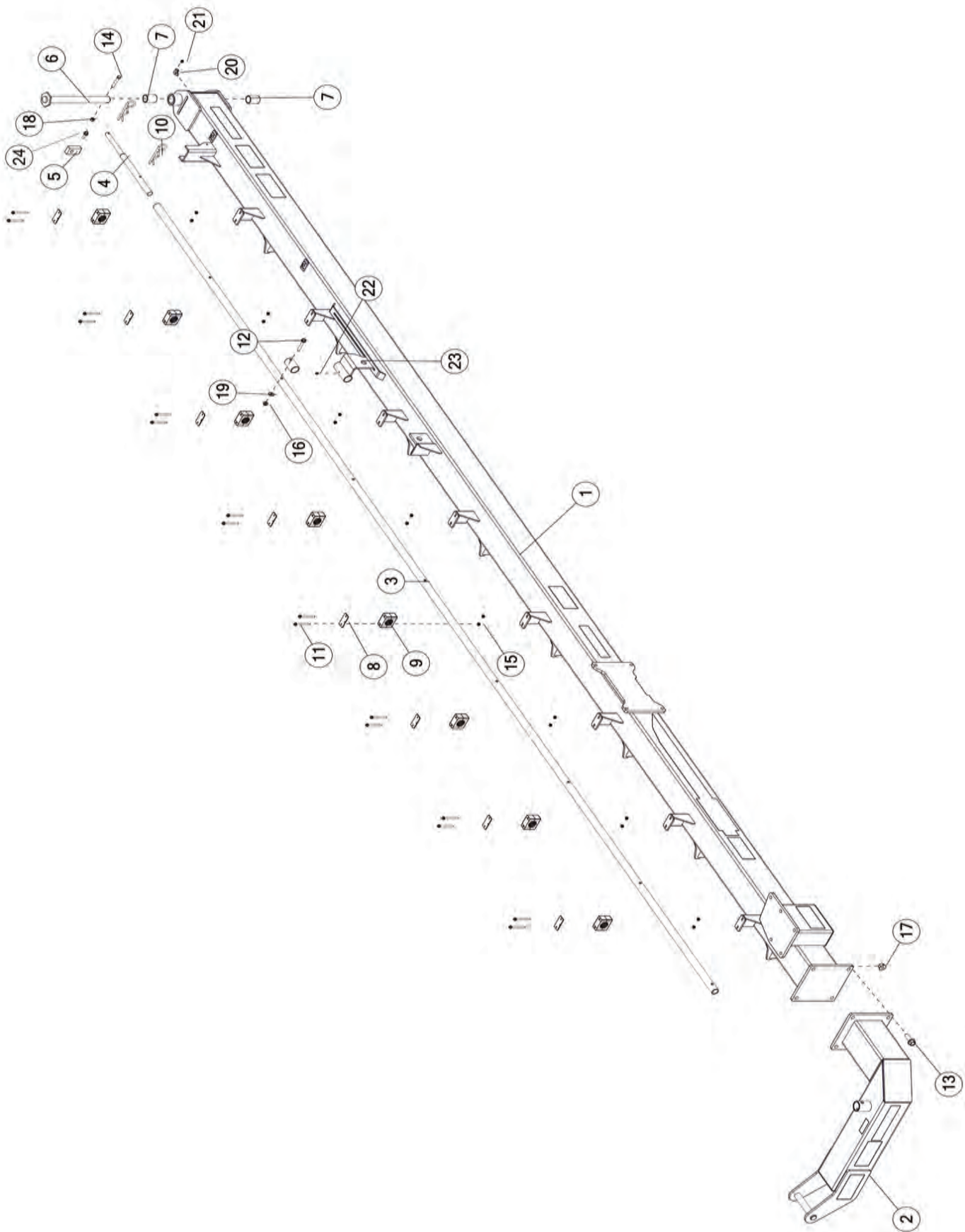
FIGURE 8 MAIN RAKE BEAM ARM LH & COMPONENTS
