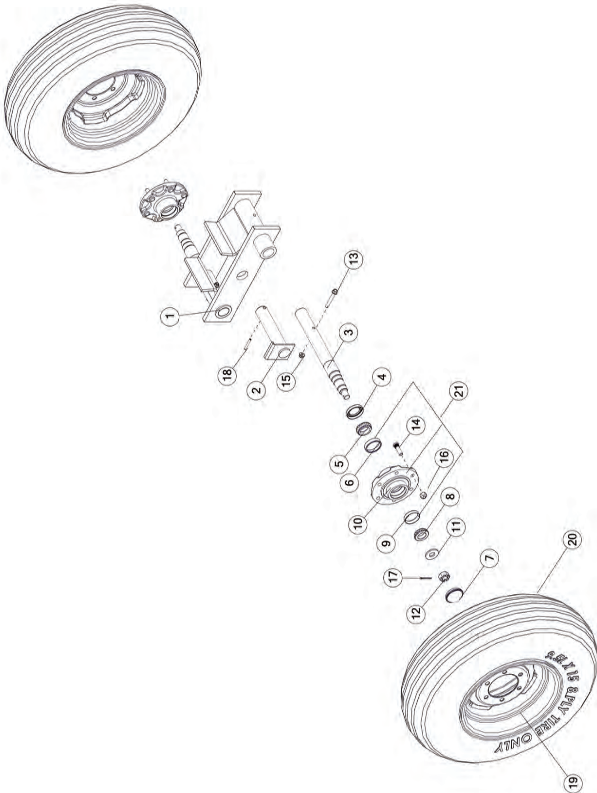
FIGURE 5 TANDEM & TIRES
