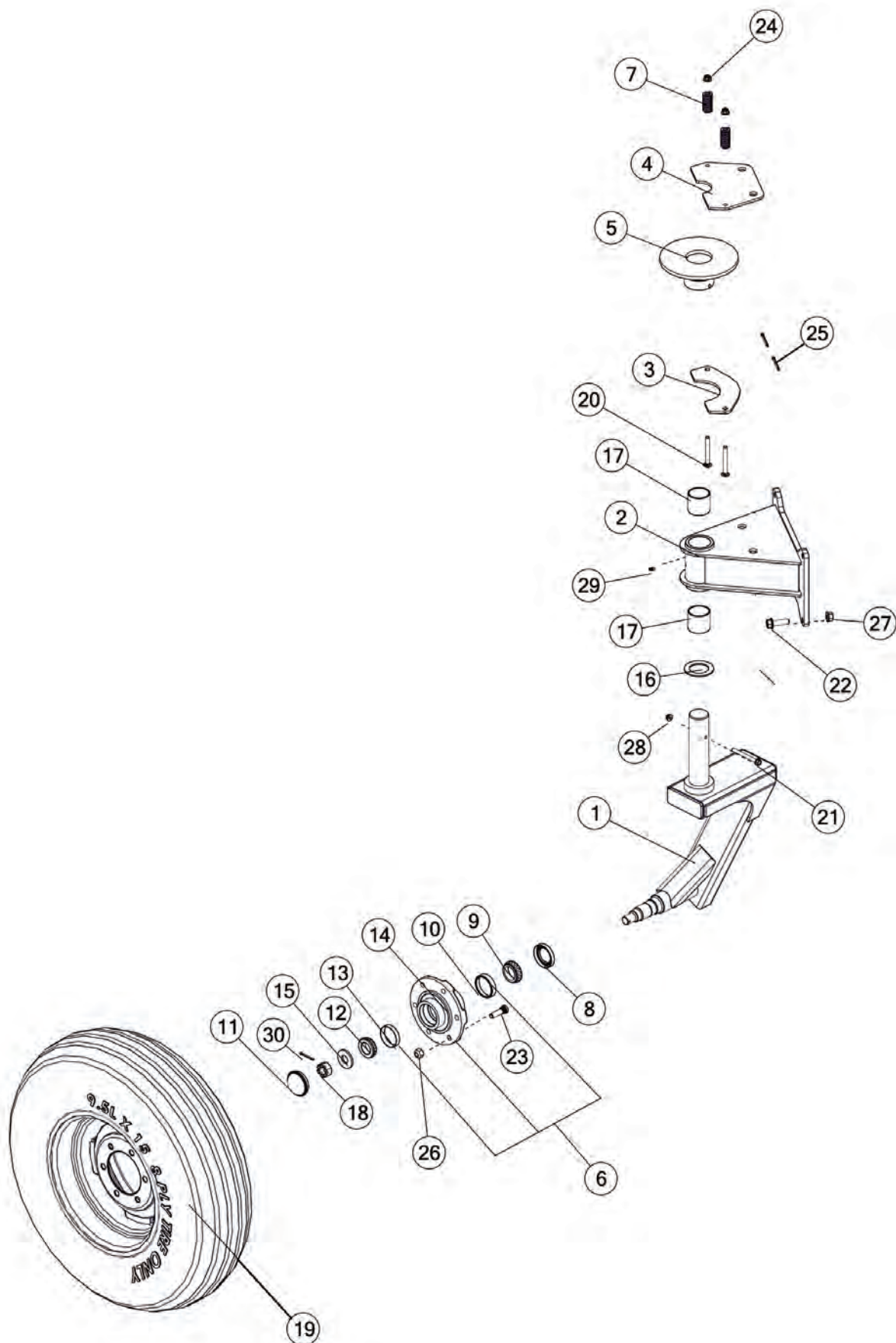
FIGURE 16 CASTER AND COMPONENT OPTIONS
