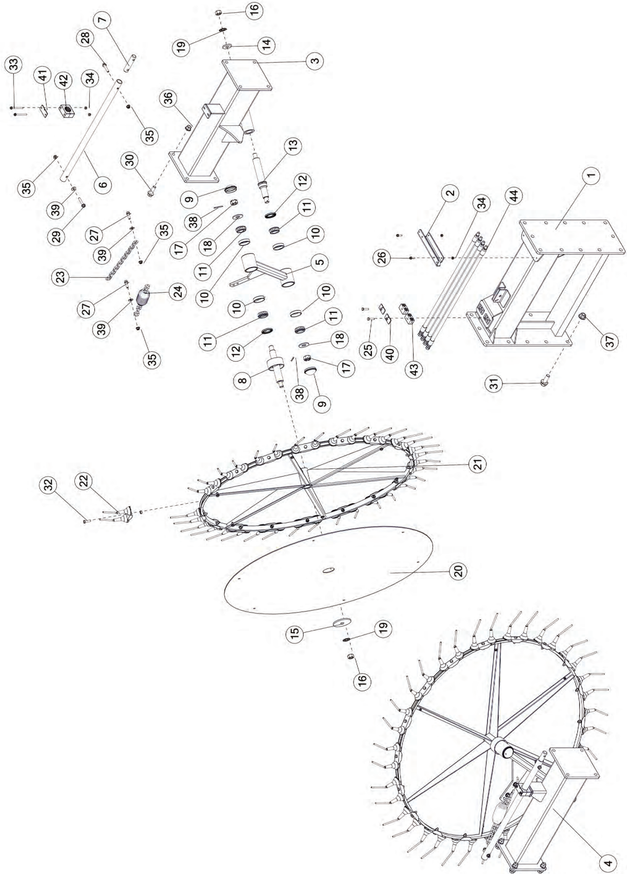
FIGURE 15 2 WHEEL EXTENSION OPTION
