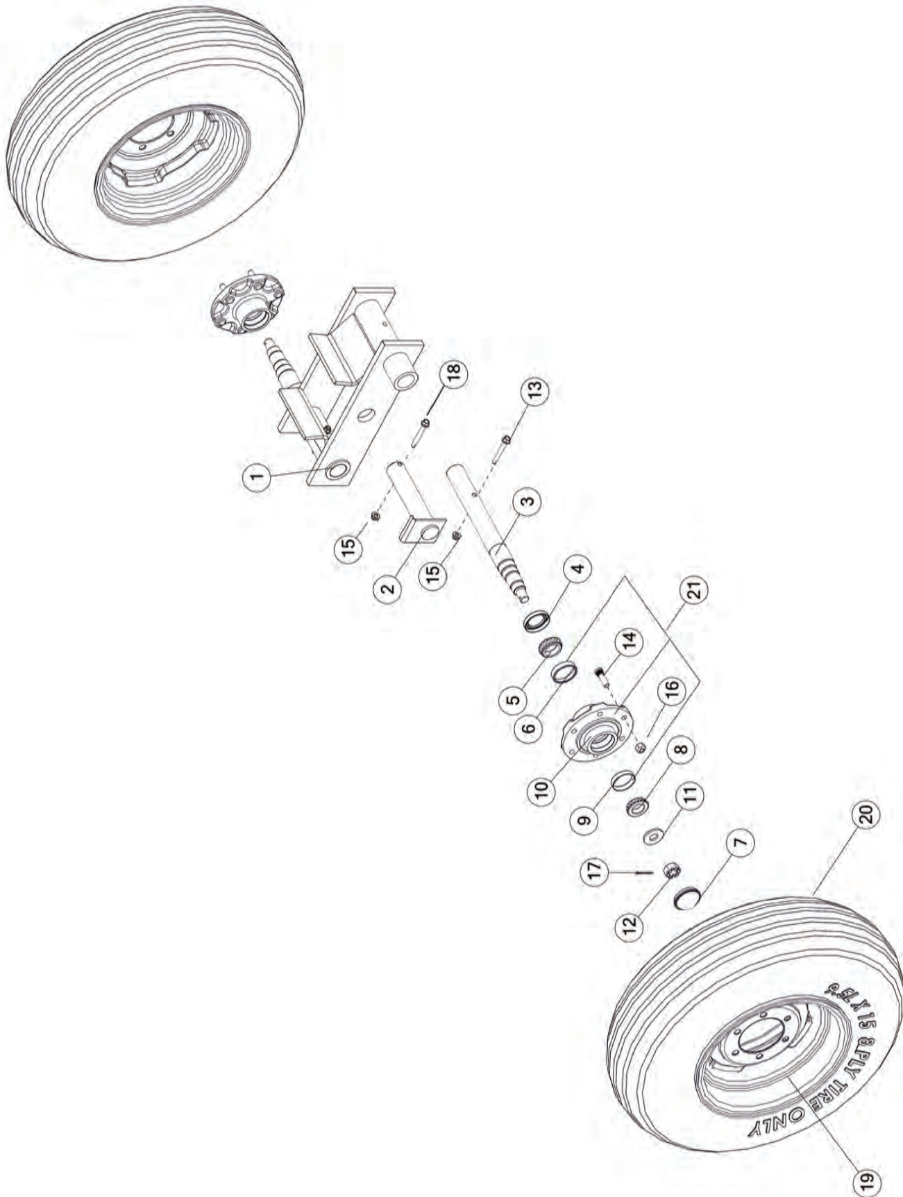
FIGURE 5 TANDEMS & TIRES
