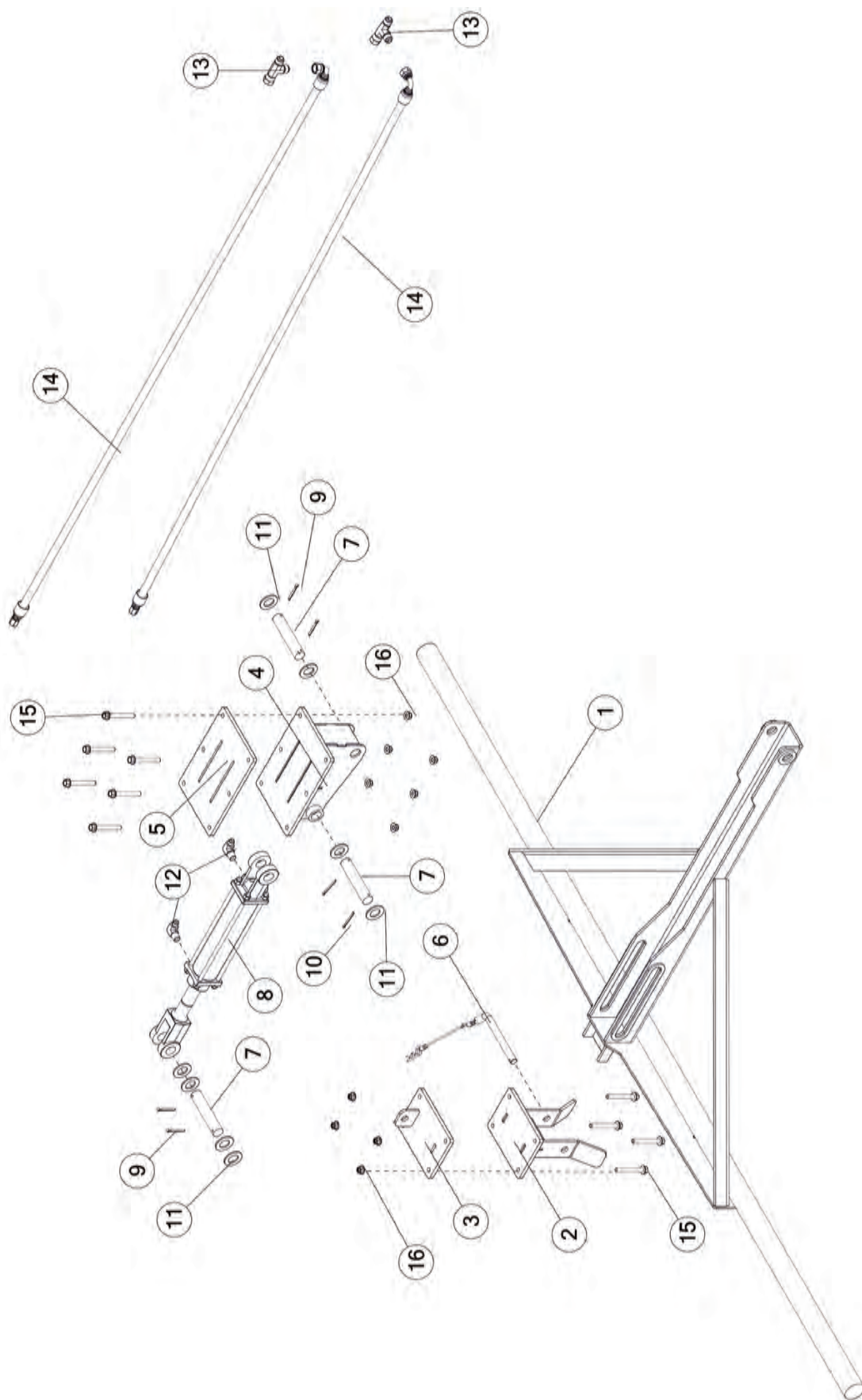
FIGURE 18 OPTIONAL CORN STALK BREAKER
