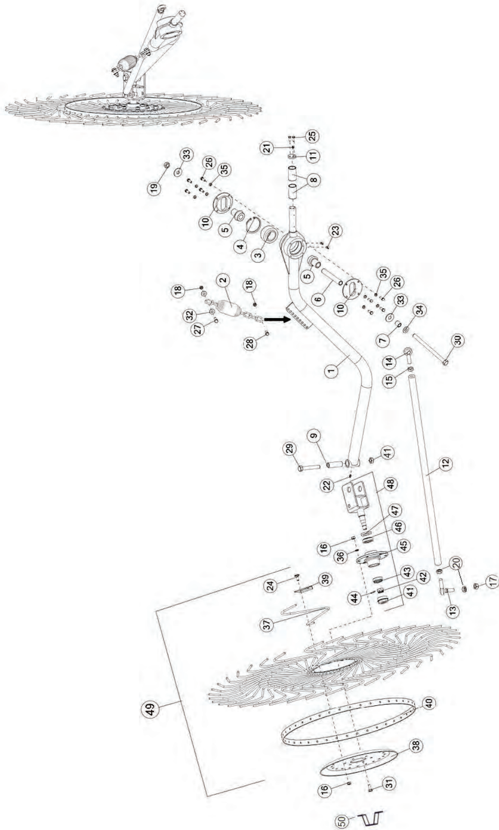
FIGURE 19 OPTIONAL KICKER WHEEL
