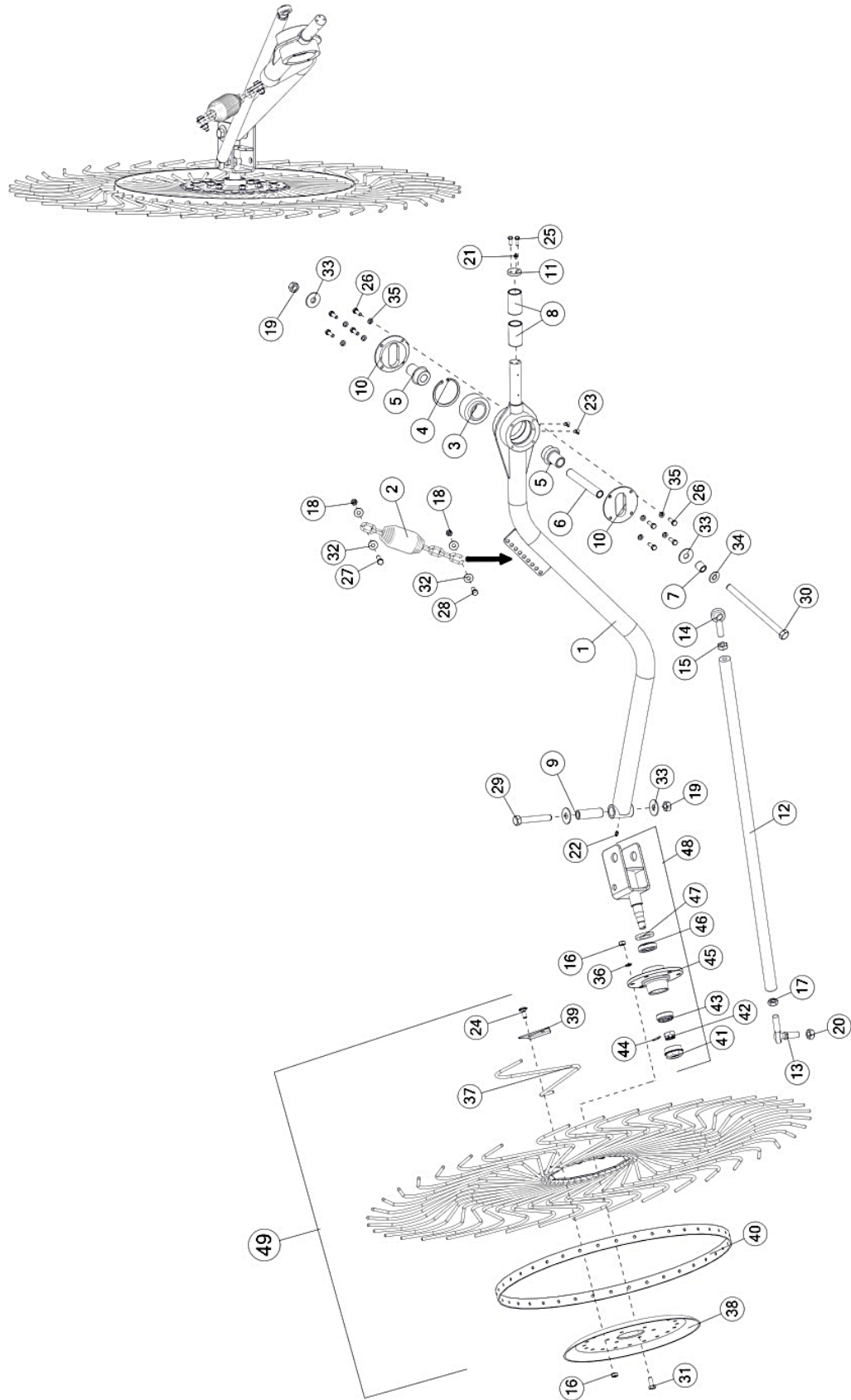
FIGURE 18 OPTIONAL KICKER WHEEL
