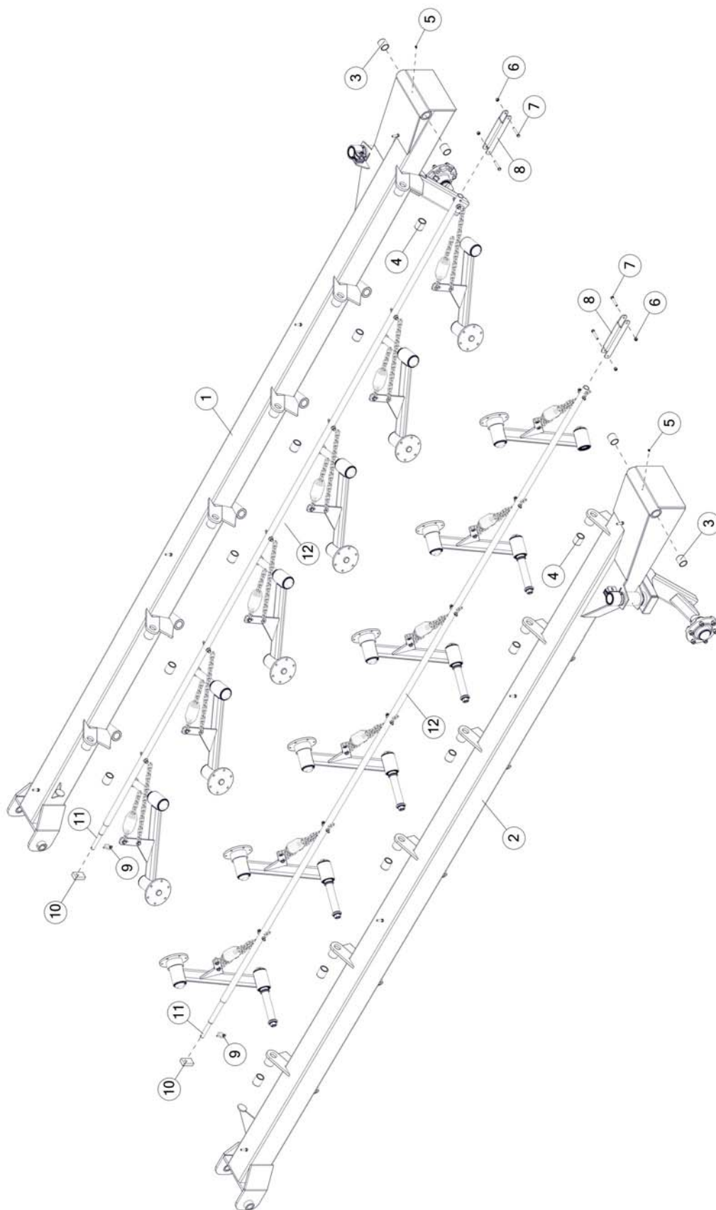
FIGURE 8 RIGHT & LEFT BACK RAKE BEAMS
