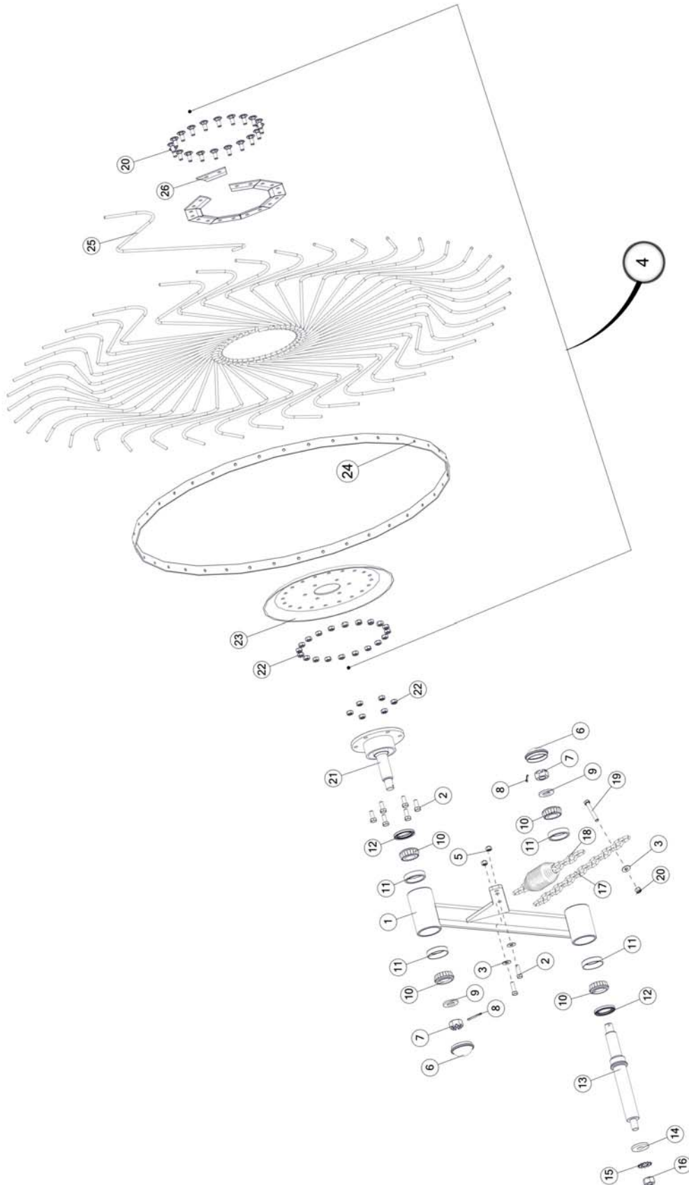
FIGURE 10 RAKE WHEEL ASSEMBLY
