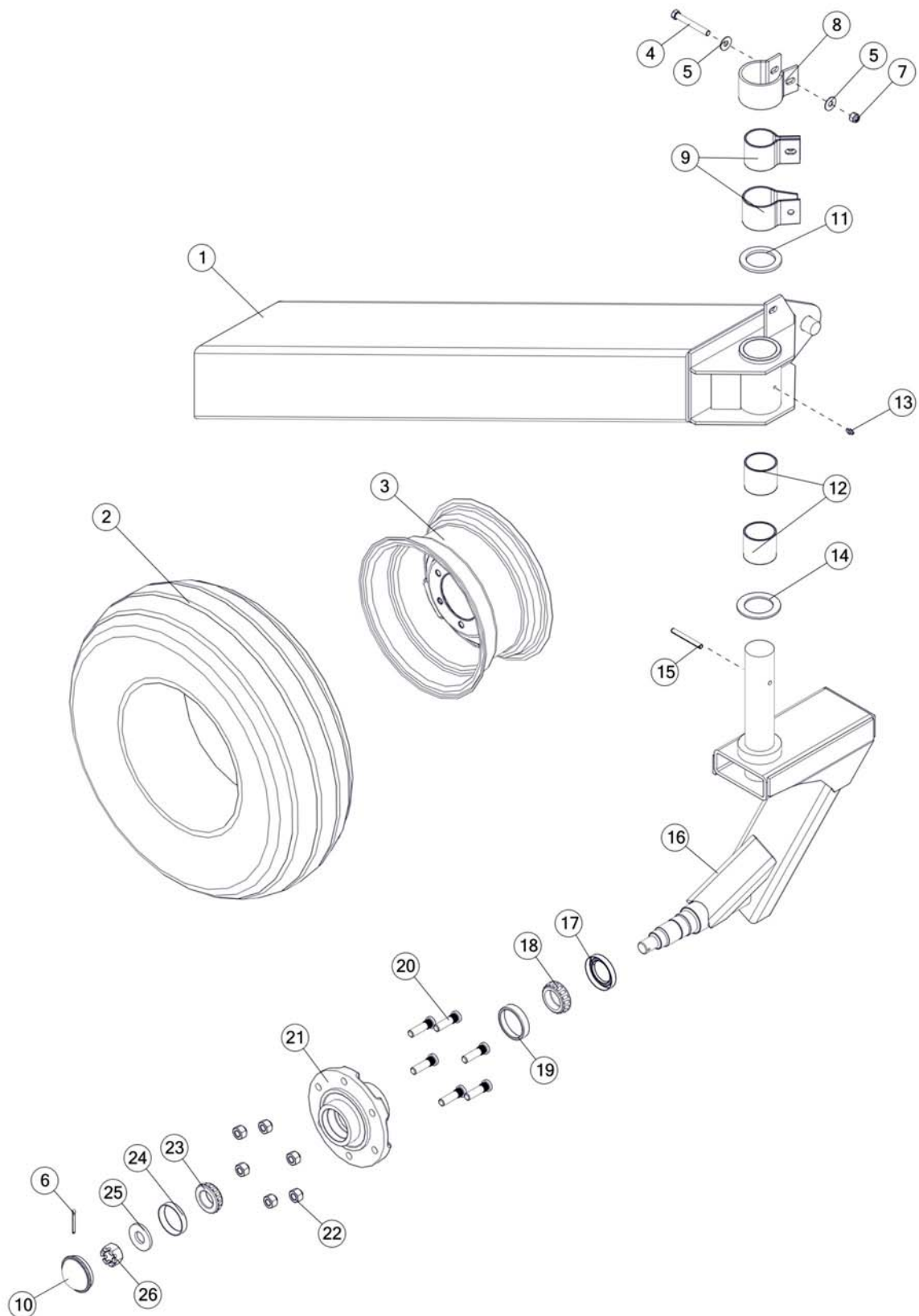
FIGURE 5 RIGHT CASTER
