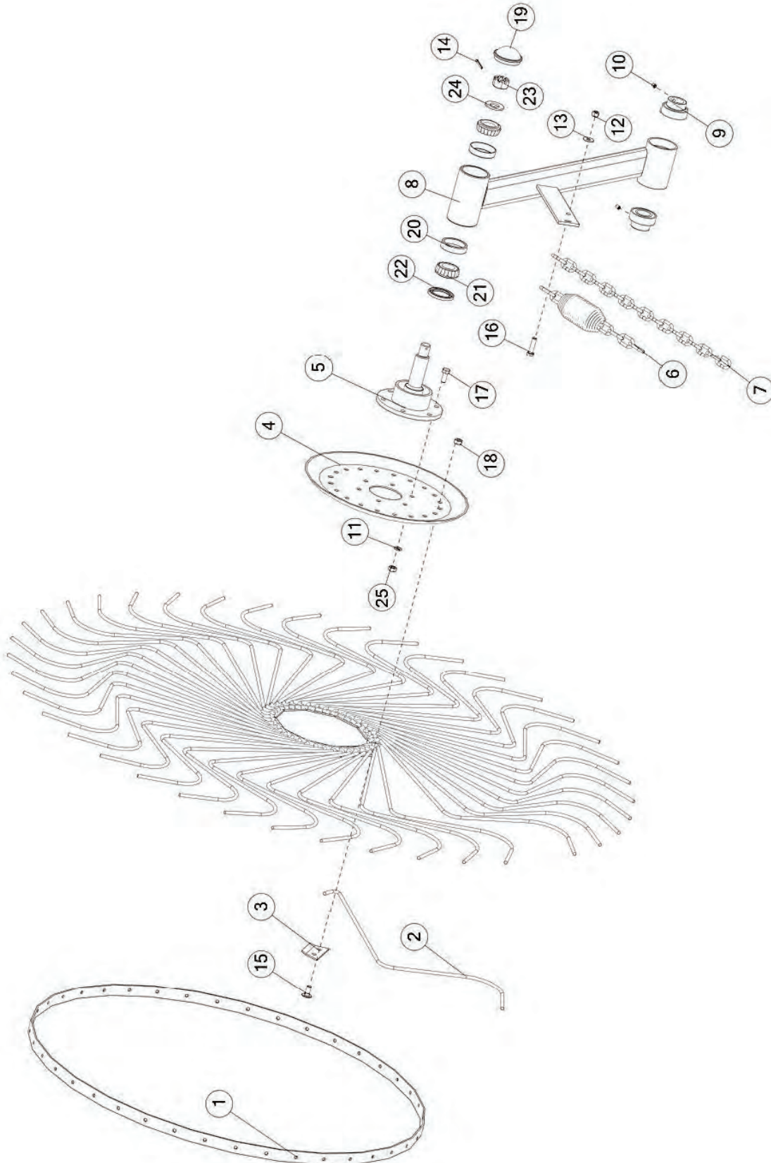
FIGURE 9 RAKE WHEEL ASSEMBLY
