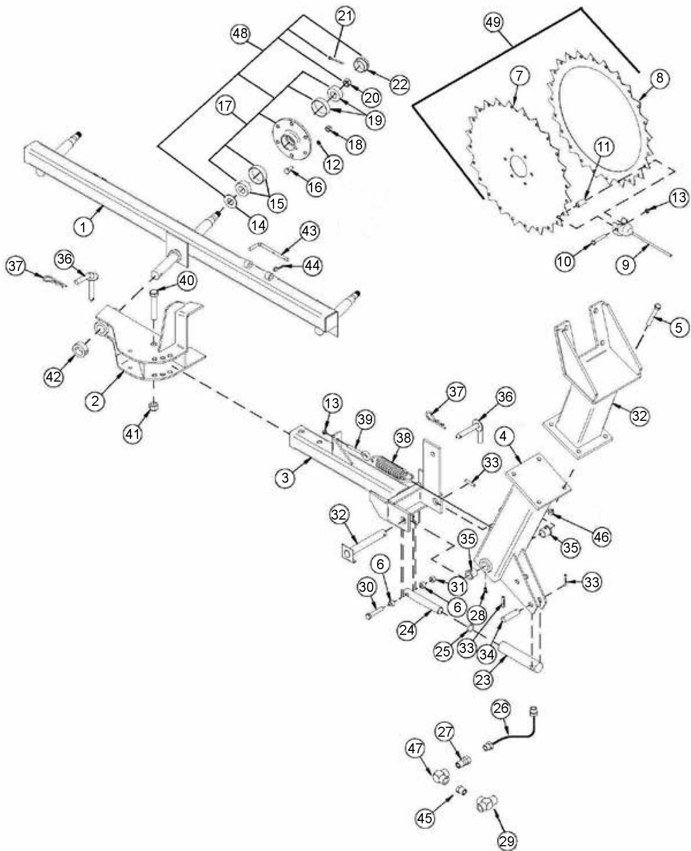
FIGURE 16 OPTIONAL 3 WHEEL CENTER KICKER WHEEL
