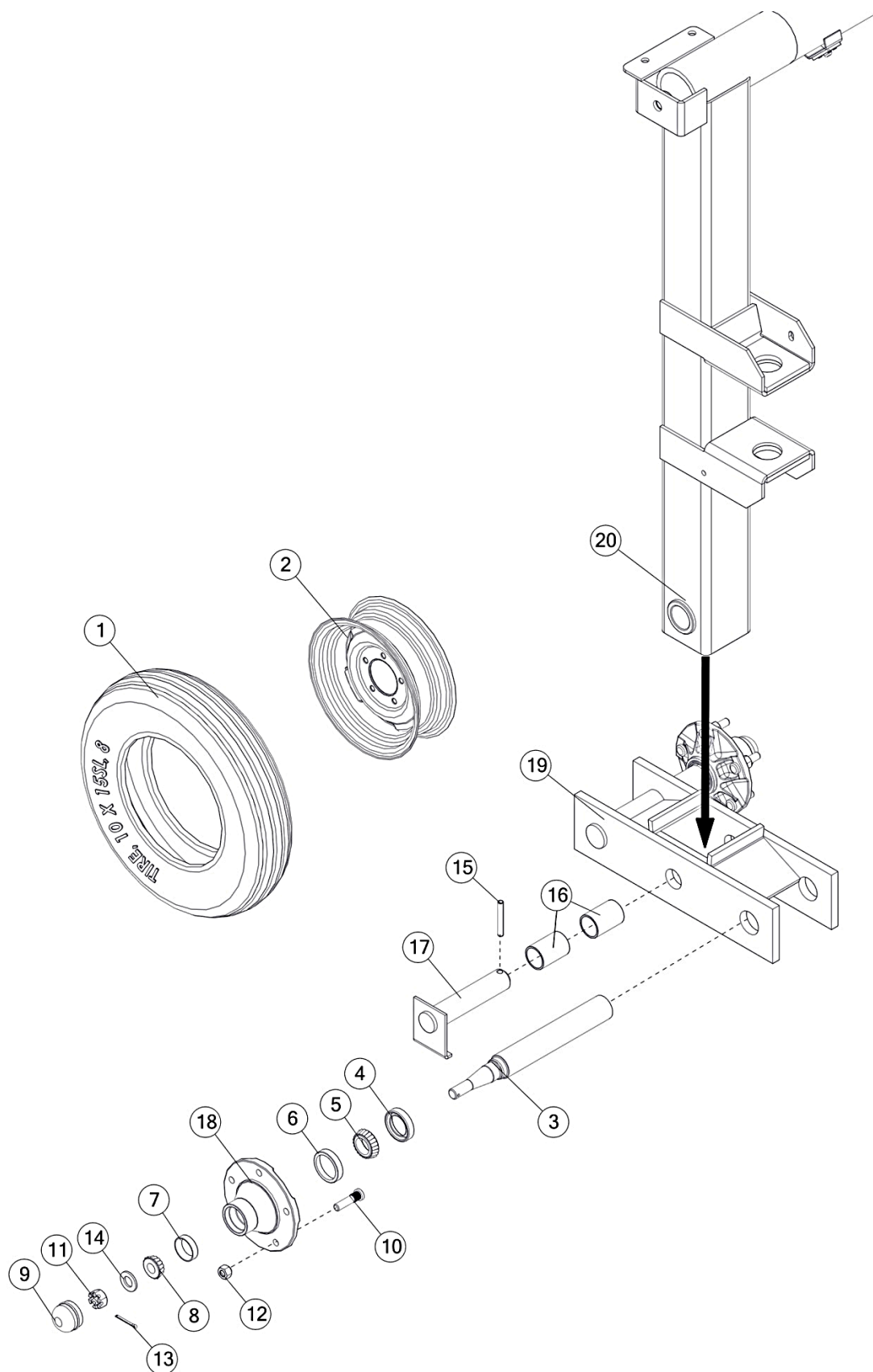
FIGURE 5 REAR HUB ASSEMBLY
