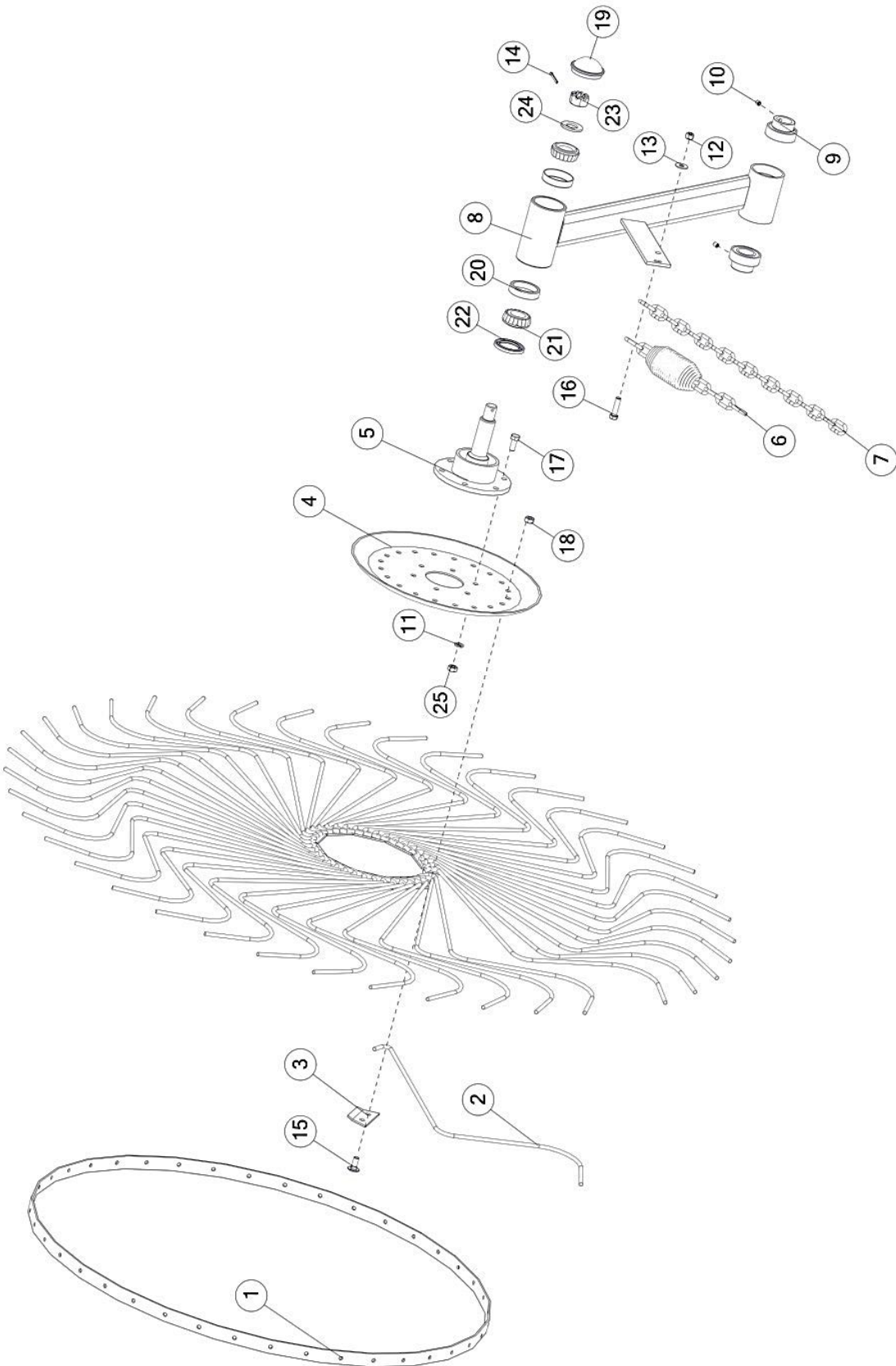
FIGURE 9 RAKE WHEEL ASSEMBLY
