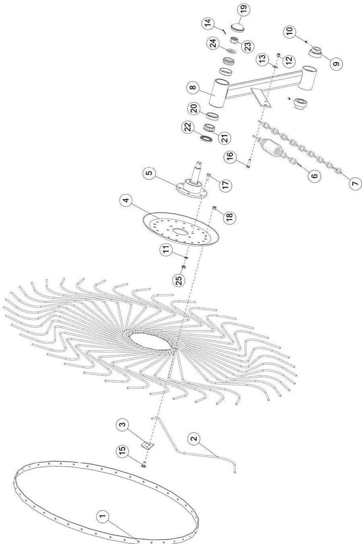
FIGURE 9 RAKE WHEEL ASSEMBLY
