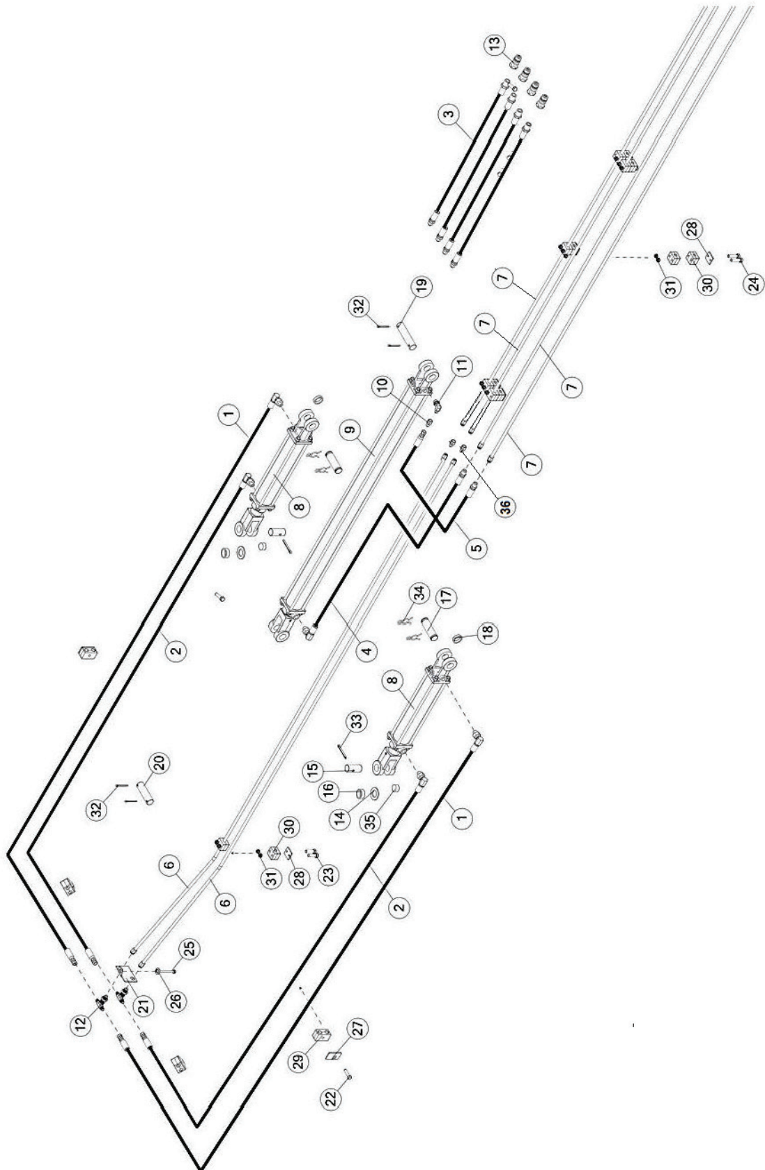
FIGURE 11 HYDRAULICS
