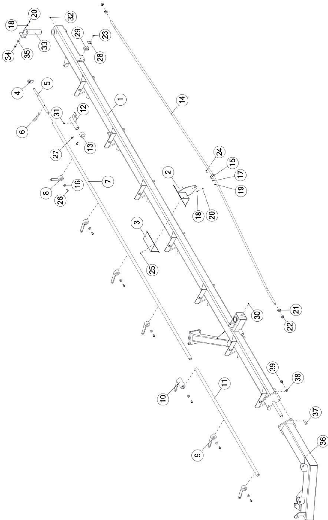
FIGURE 8 LH RAKE BEAM ASSEMBLY
