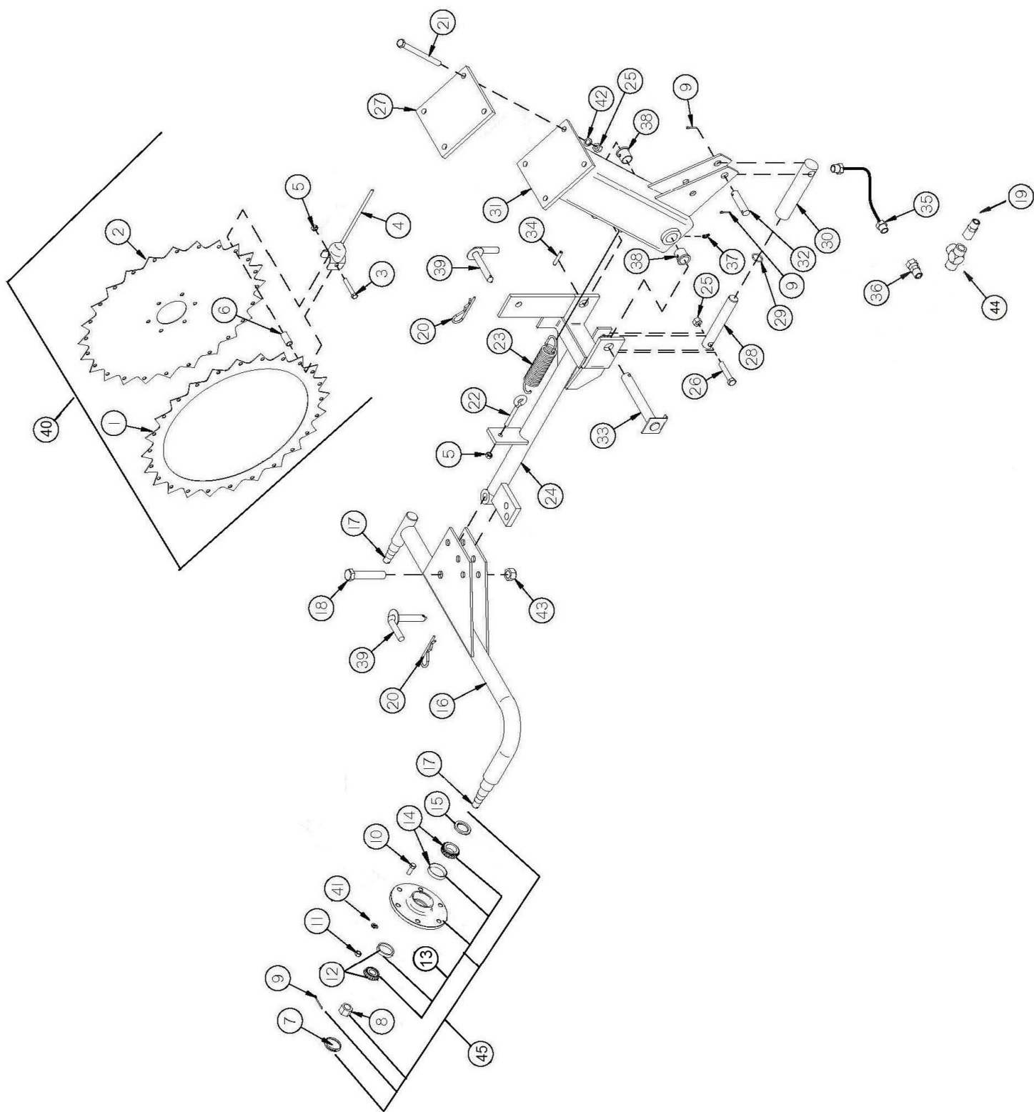
FIGURE 16 OPTIONAL 2 WHEEL CENTER KICKER WHEEL
