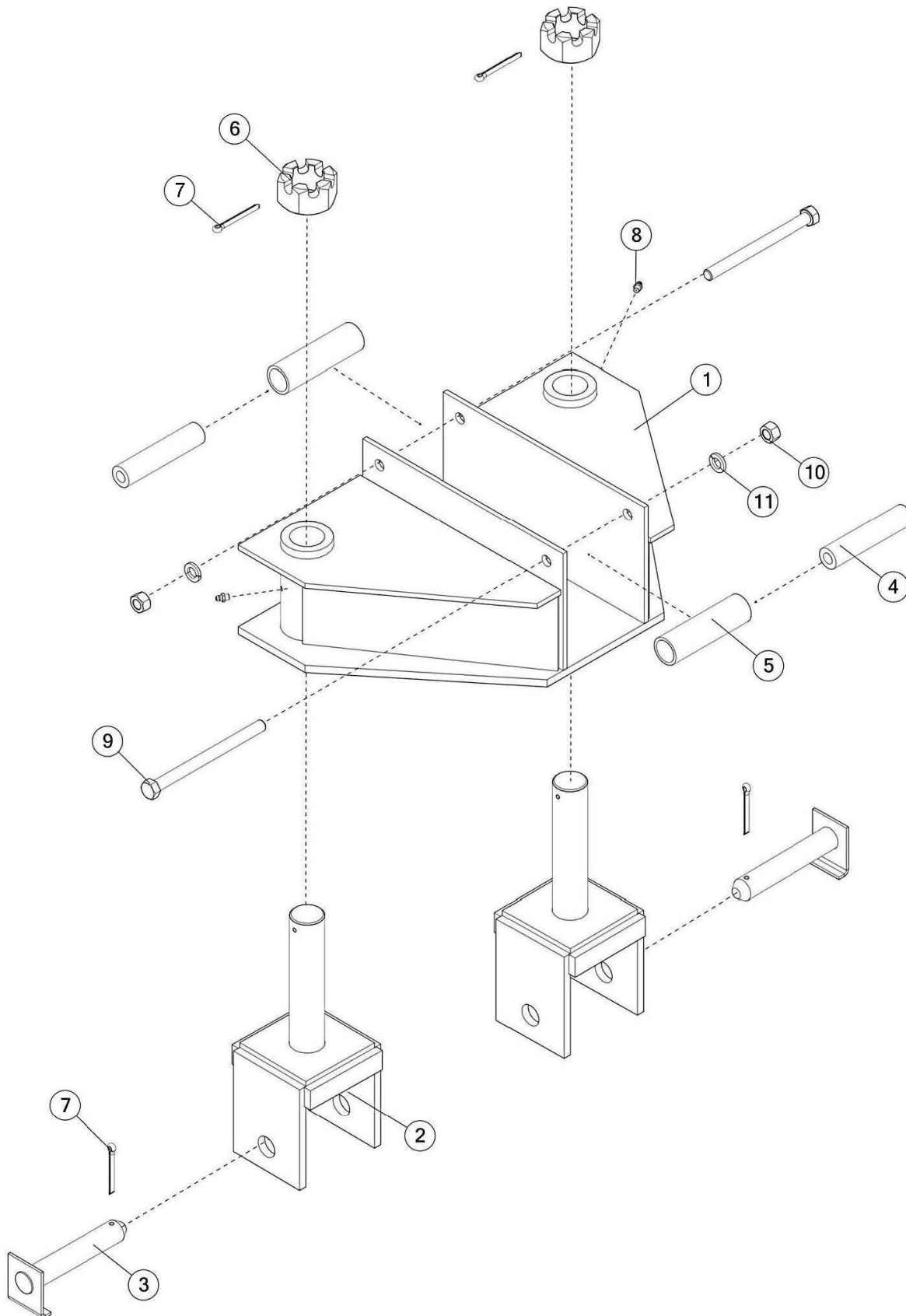
FIGURE 3 BACK LINKAGE ASSEMBLY
