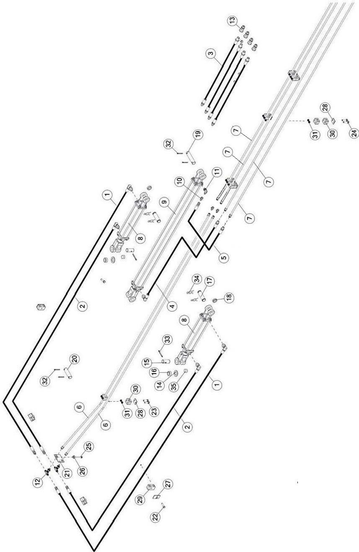
FIGURE 11 HYDRAULICS
