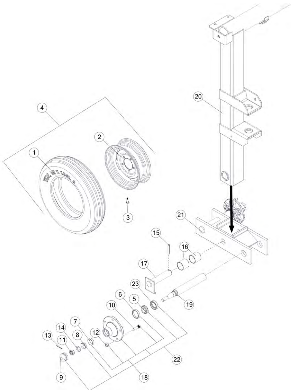
FIGURE 5 REAR HUB ASSEMBLY
