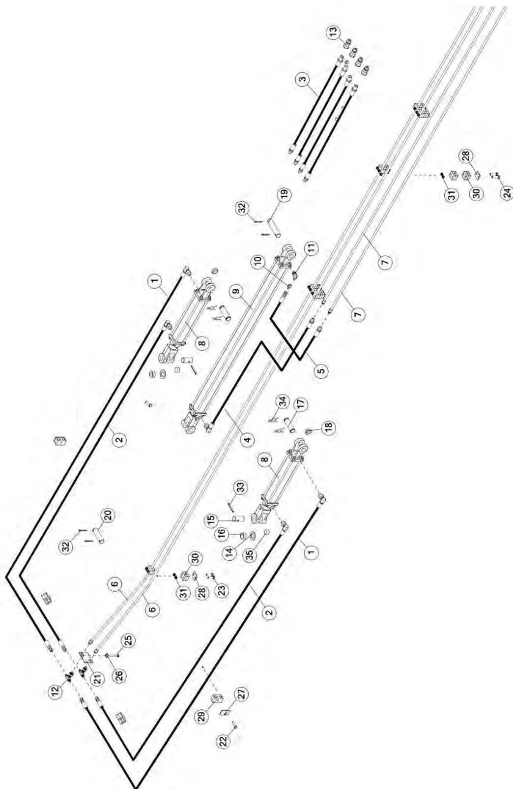
FIGURE 11 HYDRAULICS
