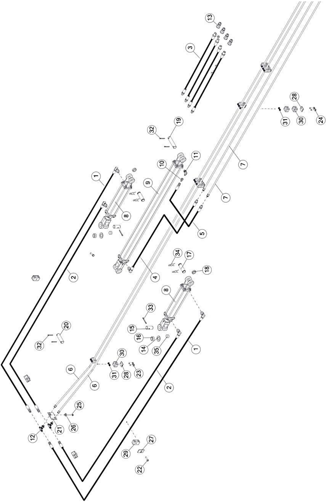
FIGURE 11 HYDRAULICS
