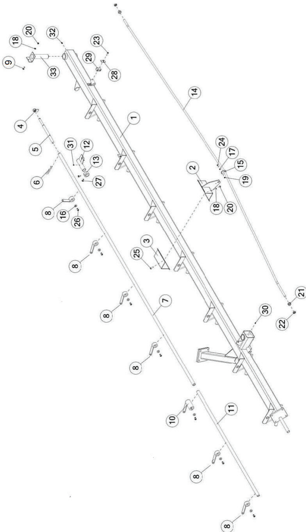
FIGURE 8 LH RAKE BEAM ASSEMBLY
