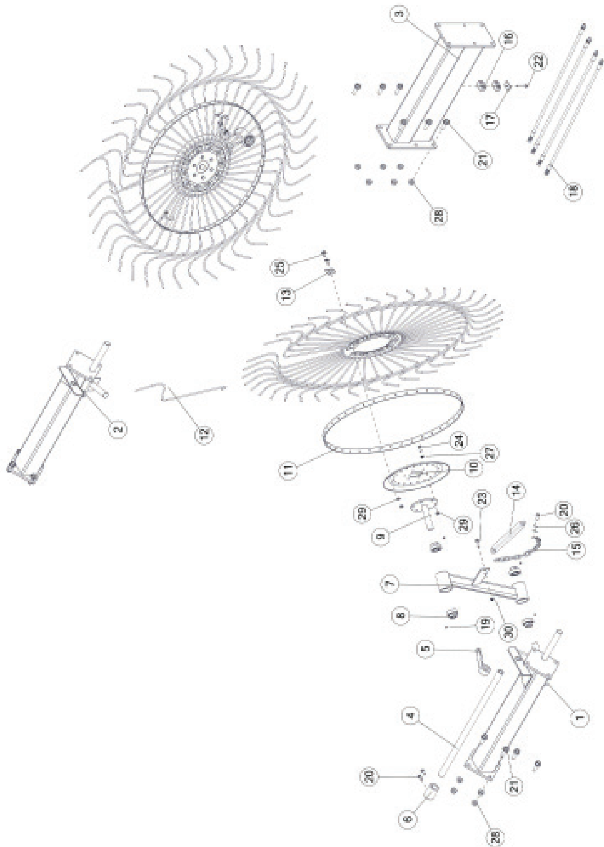
FIGURE 15 OPTIONAL 2 WHEEL EXTENSION
