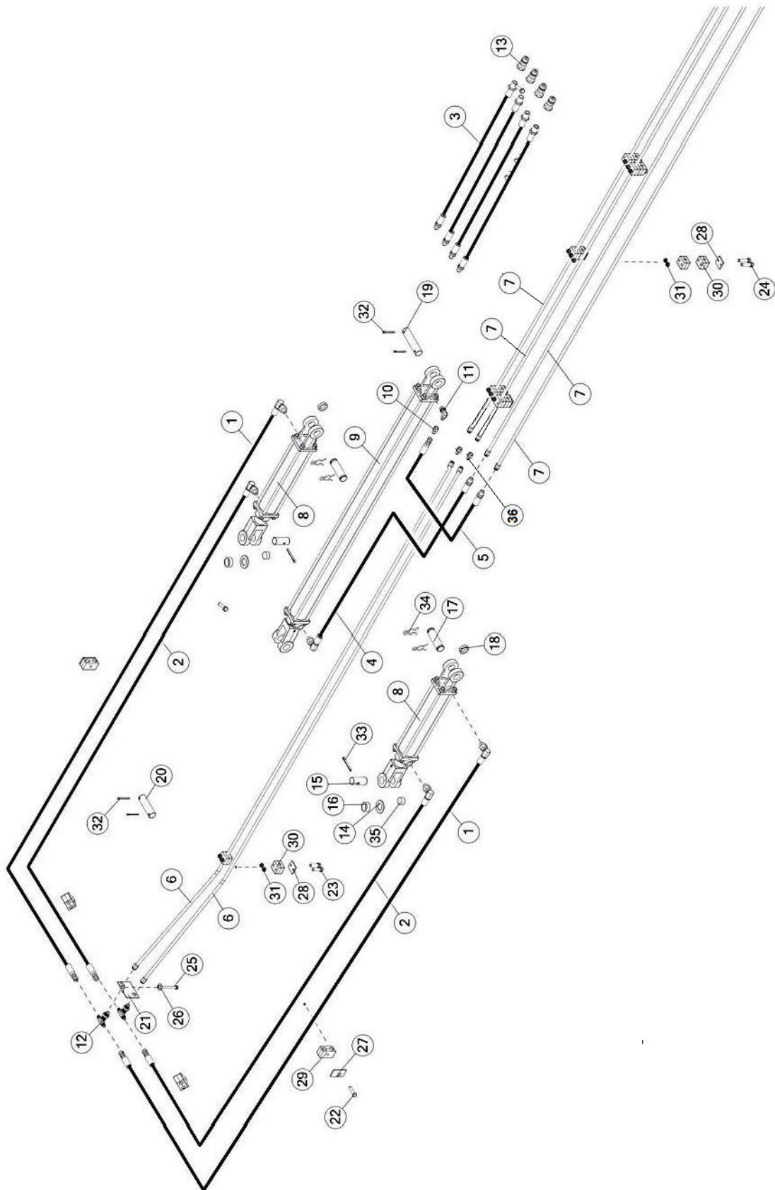
FIGURE 11 HYDRAULICS
