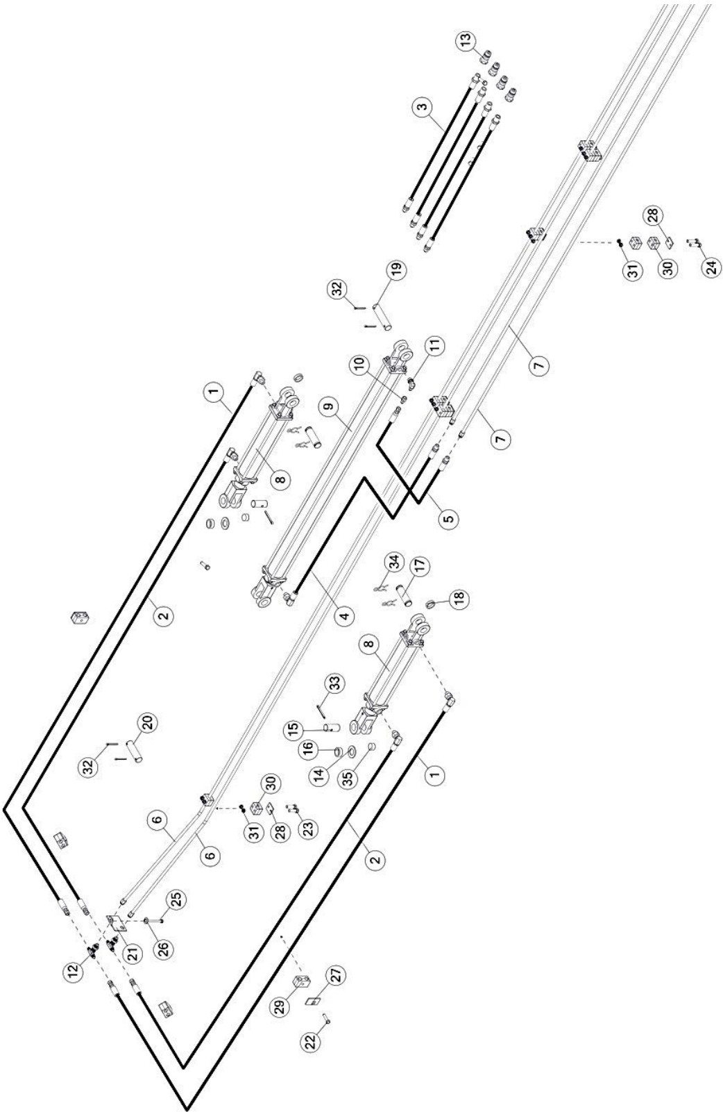
FIGURE 11 HYDRAULICS
