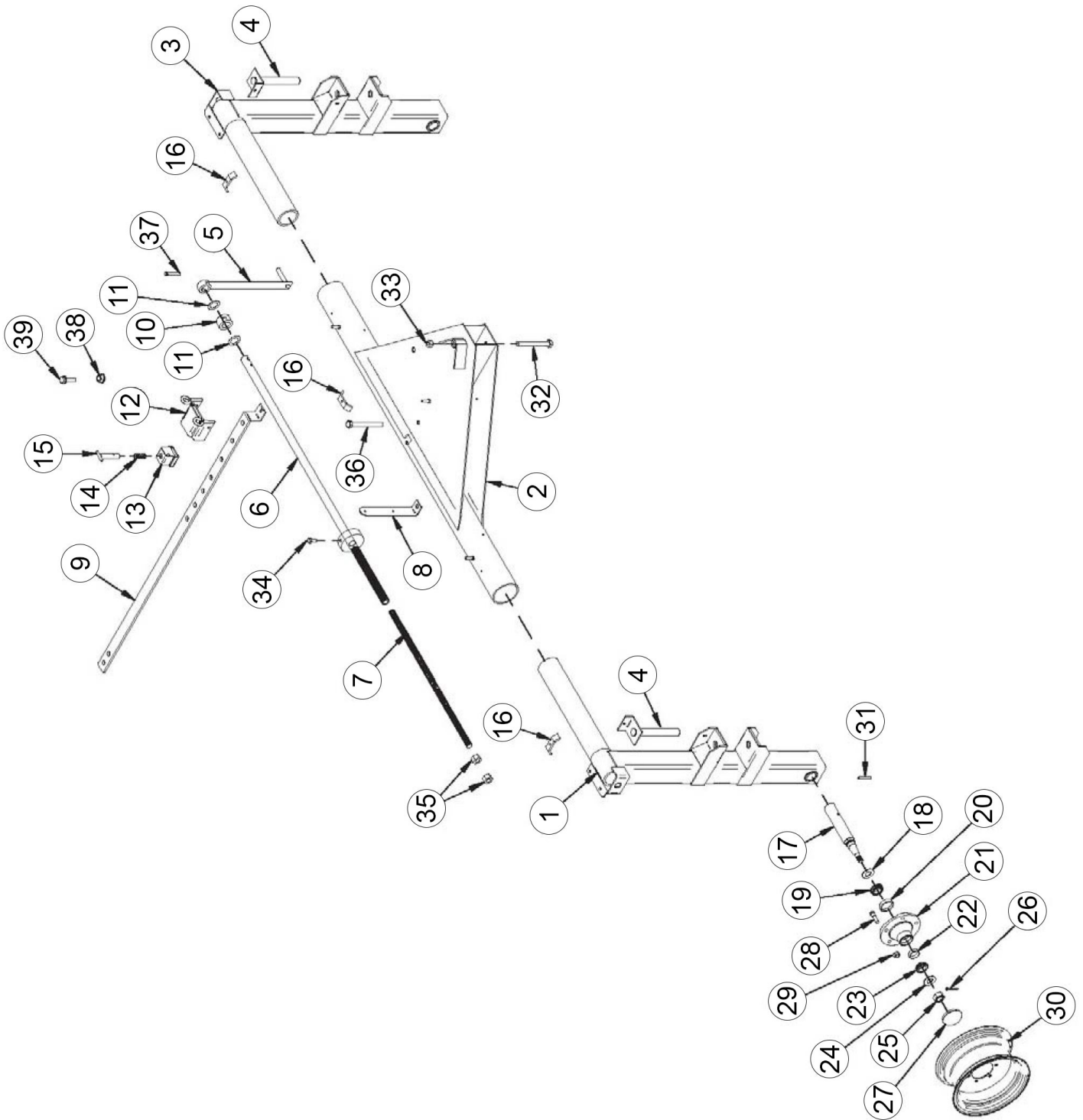
FIGURE 1 MAIN FRAME REAR
