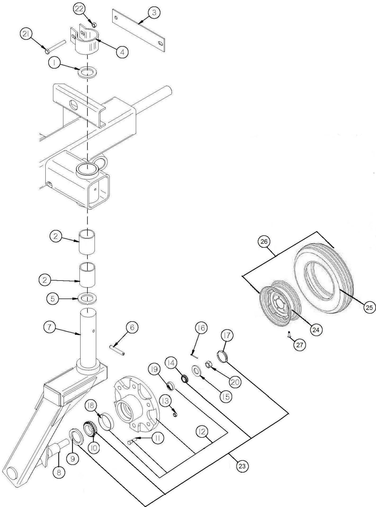
FIGURE 4 GAUGE WHEEL
