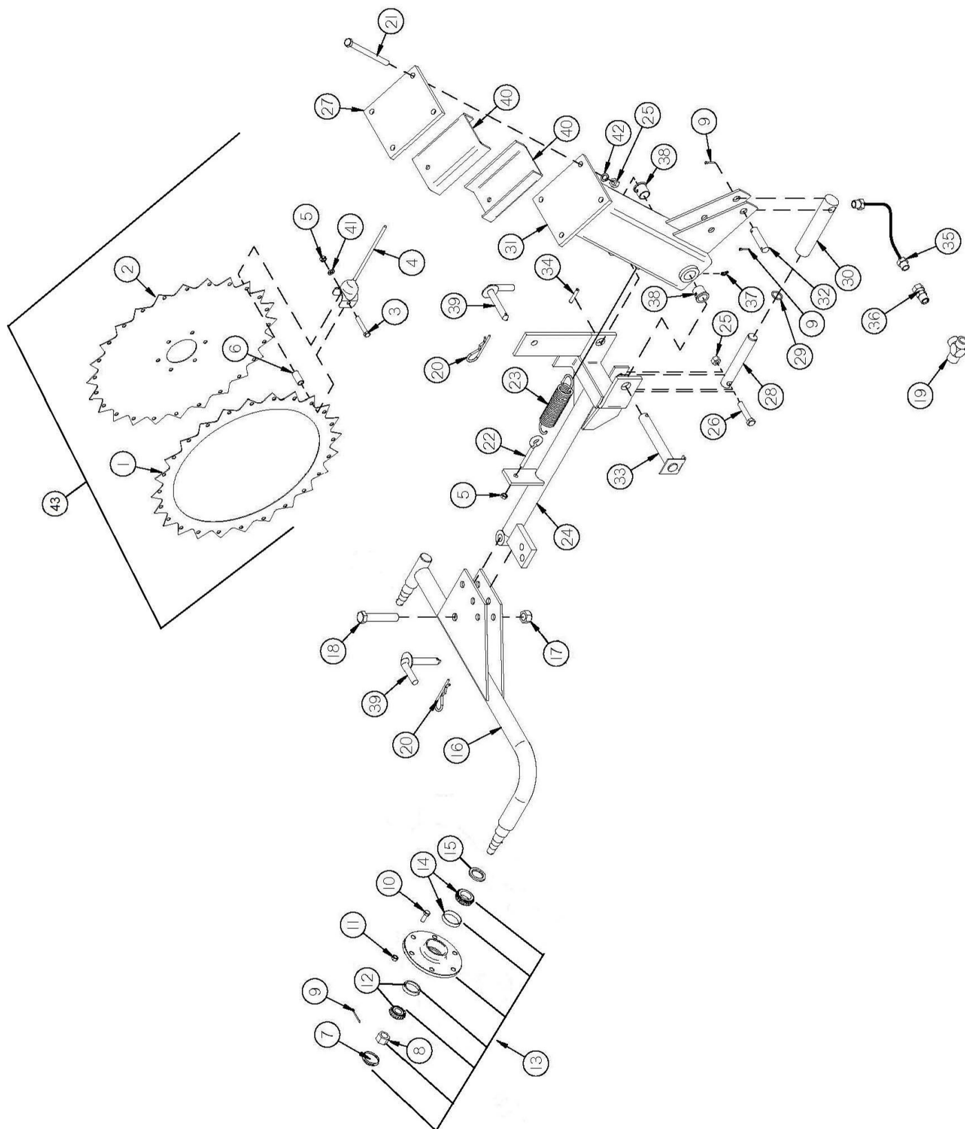
FIGURE 8 OPTIONAL 2 WHEEL CENTER KICKER WHEEL
