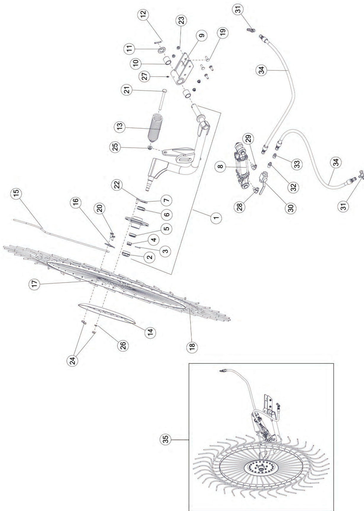
FIGURE 10 OPTIONAL CENTER KICKER WHEEL (ARO2CKW)
