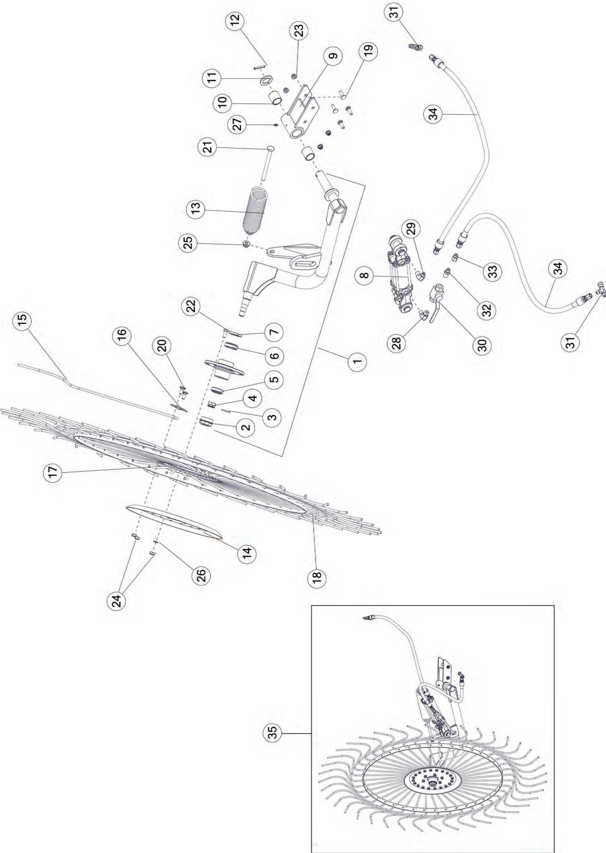
FIGURE 10 OPTIONAL CENTER KICKER WHEEL (ARO2CKW)
