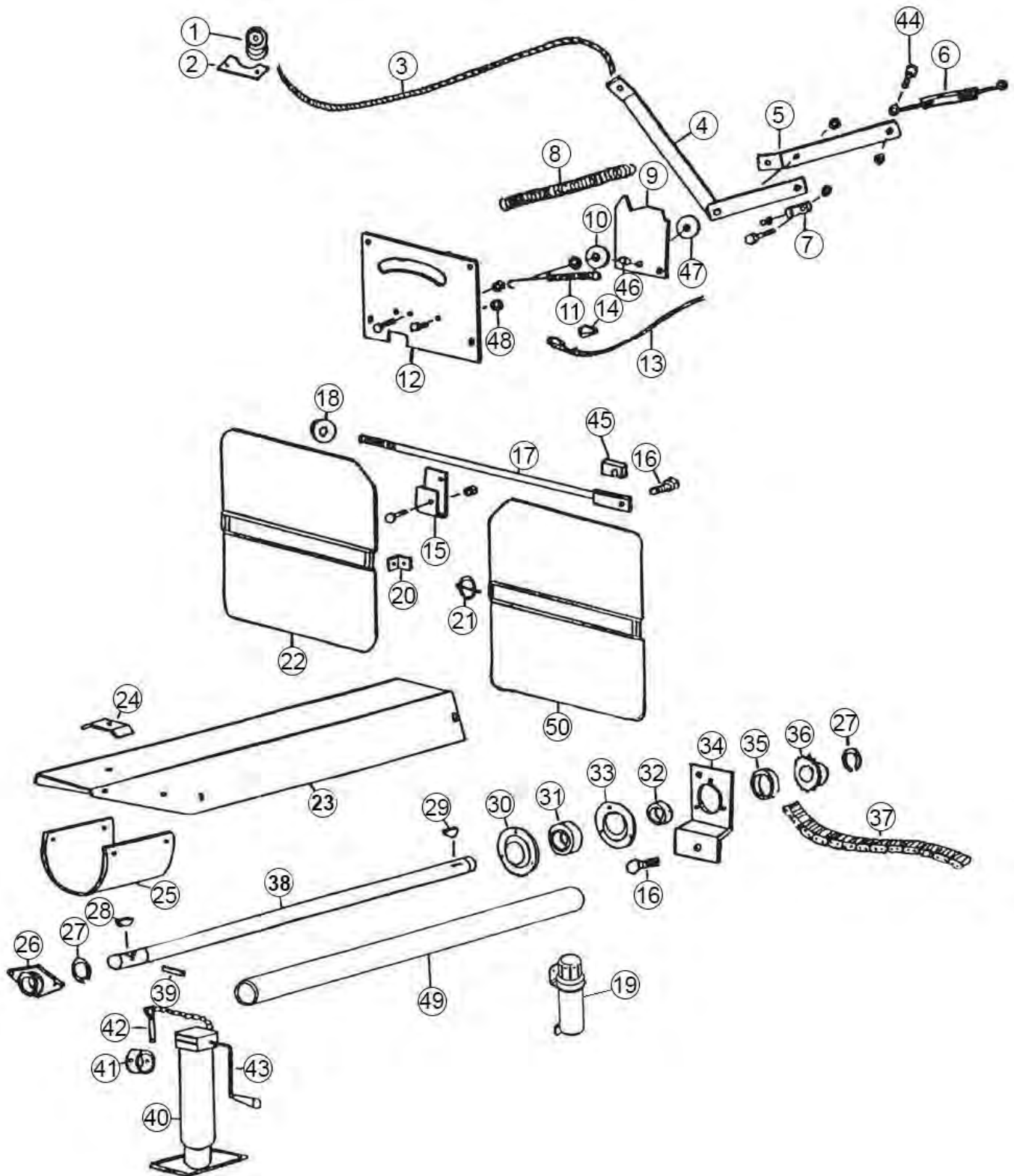
FIGURE 3 FRONT SHIELDS/DRIVE ASSEMBLY
