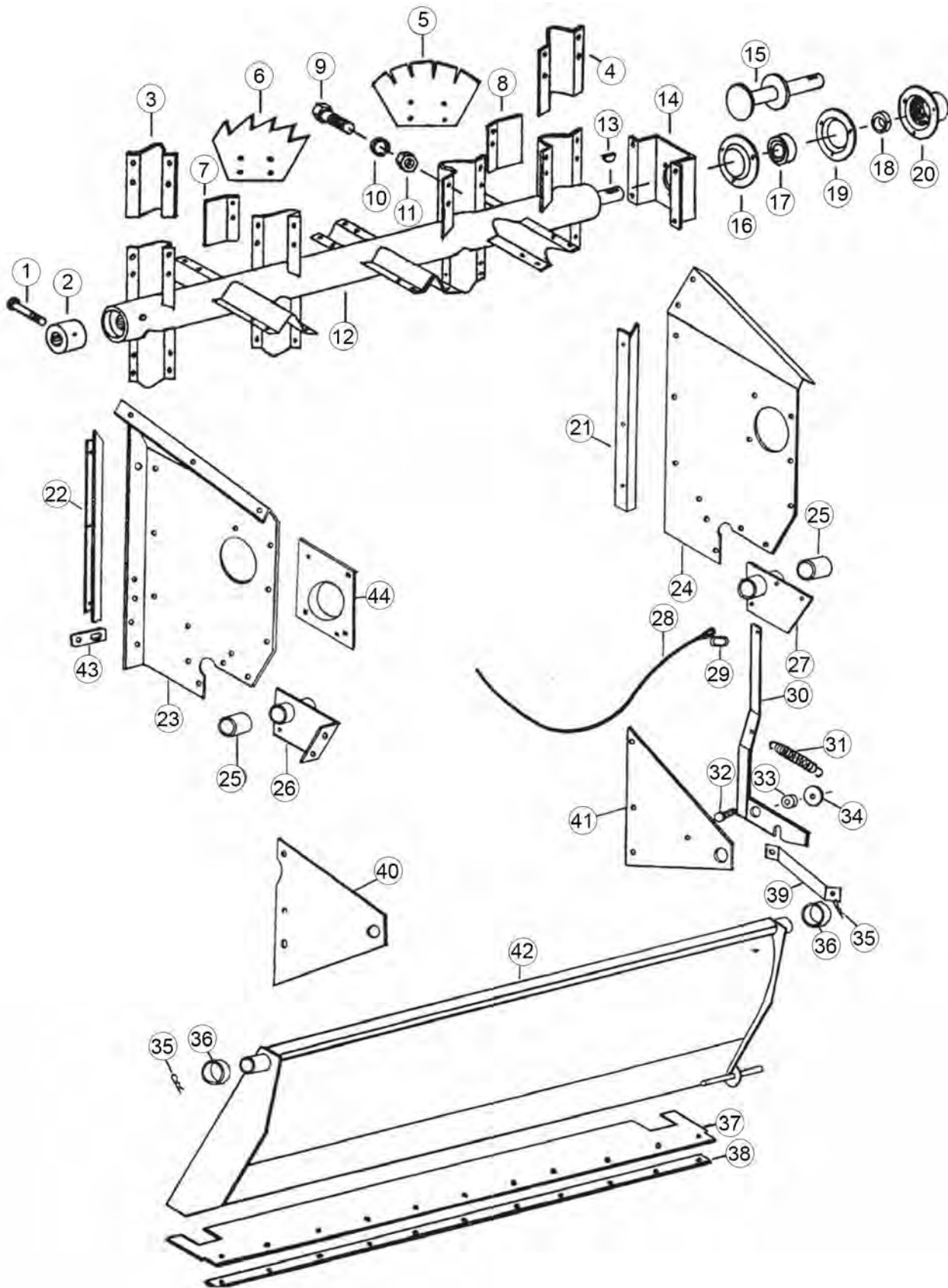
FIGURE 1 BEATER/PAN ASSEMBLY
