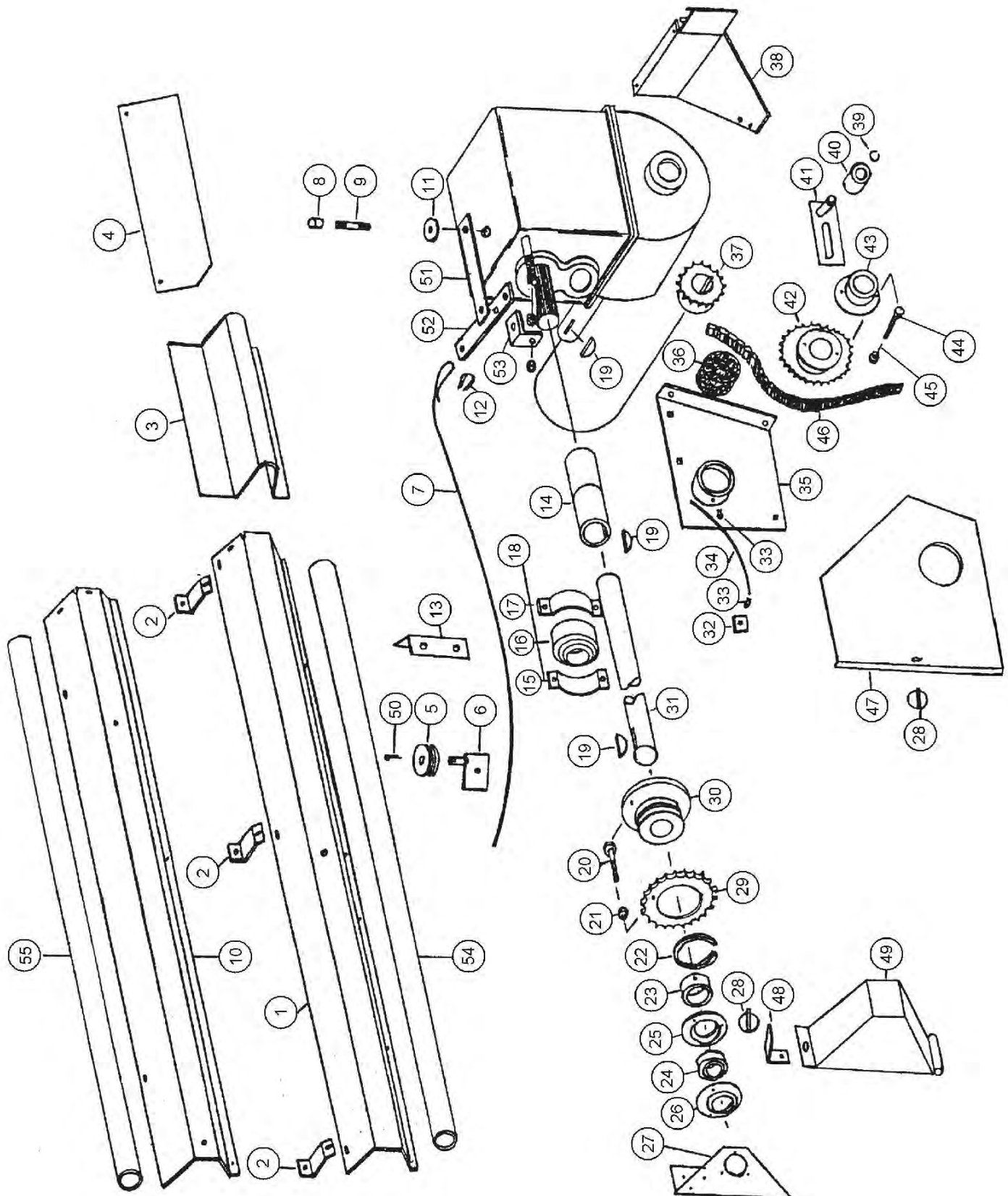
FIGURE 4 BACK SHIELDS/DRIVE ASSEMBLY
