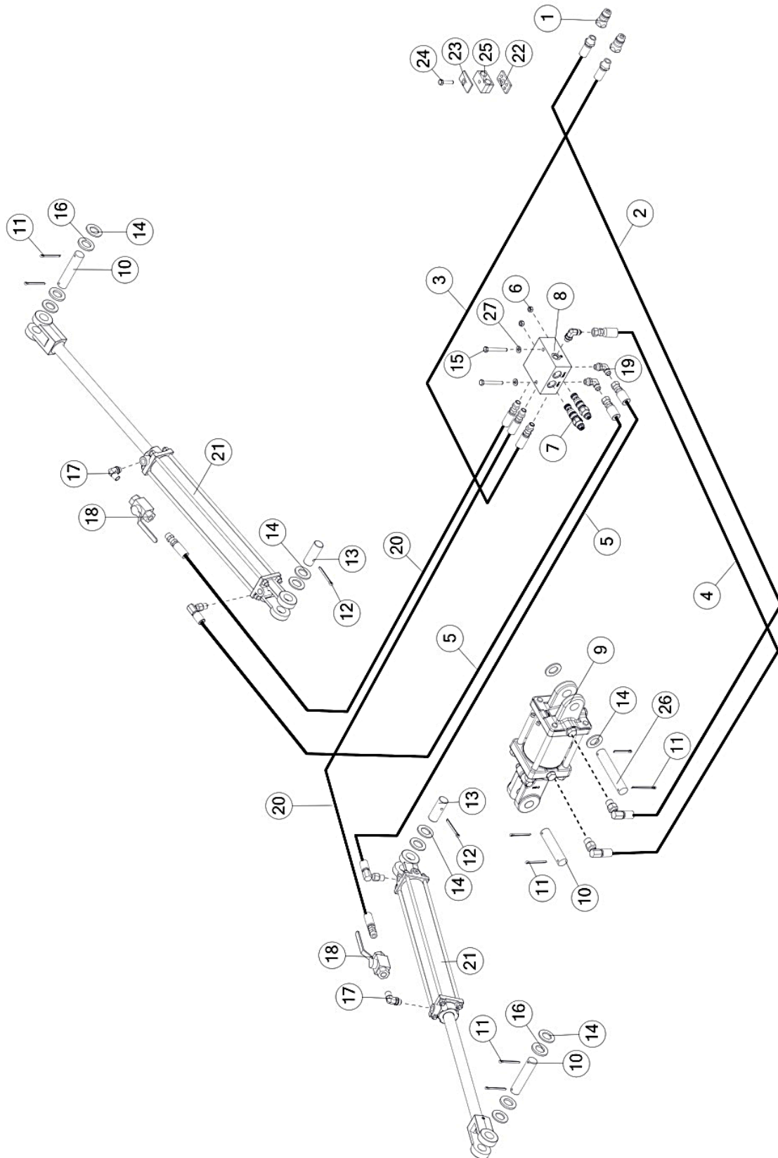
FIGURE 7 HYDRAULICS
