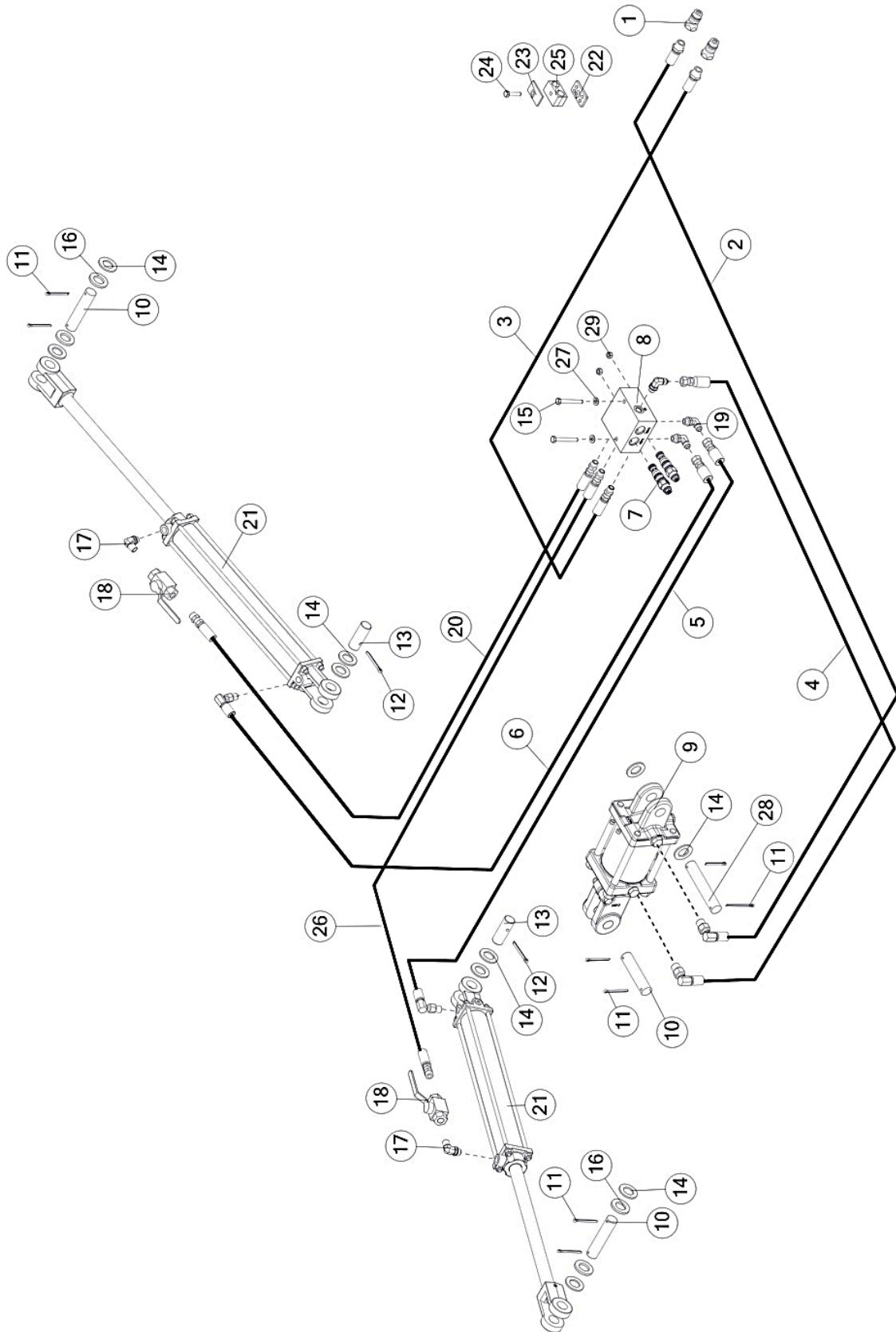
FIGURE 7 HYDRAULICS
