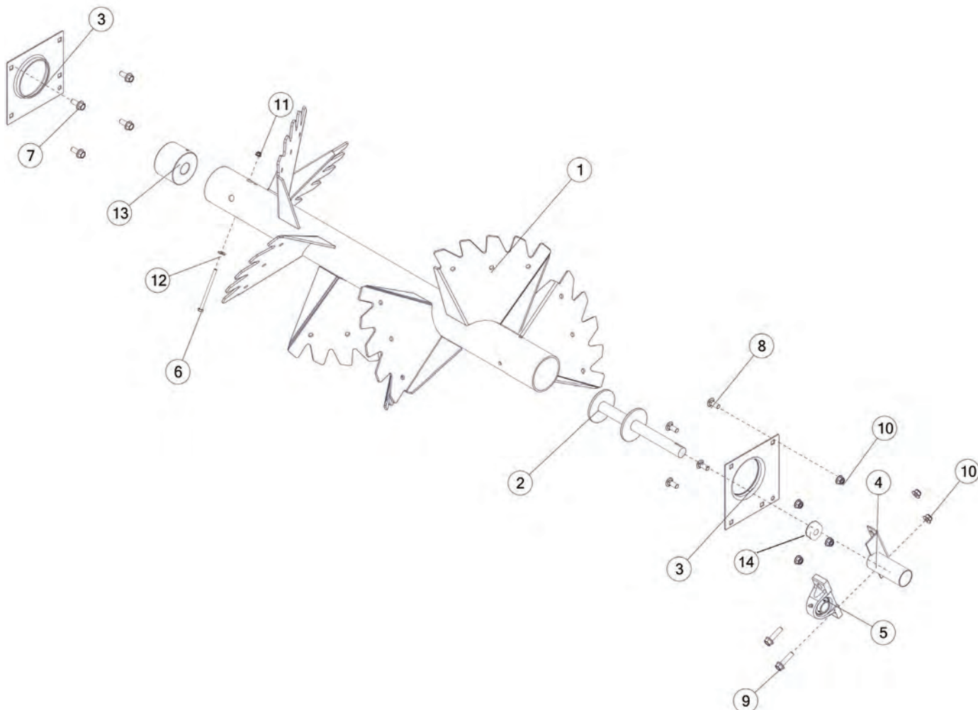
FIGURE 9 BEATER & COMPONENTS
