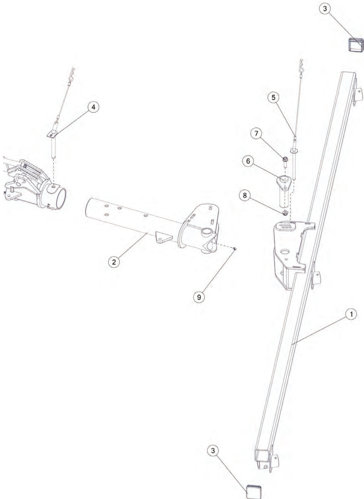
FIGURE 4 LIFT ARM PIVOT & COMPONENTS LH
