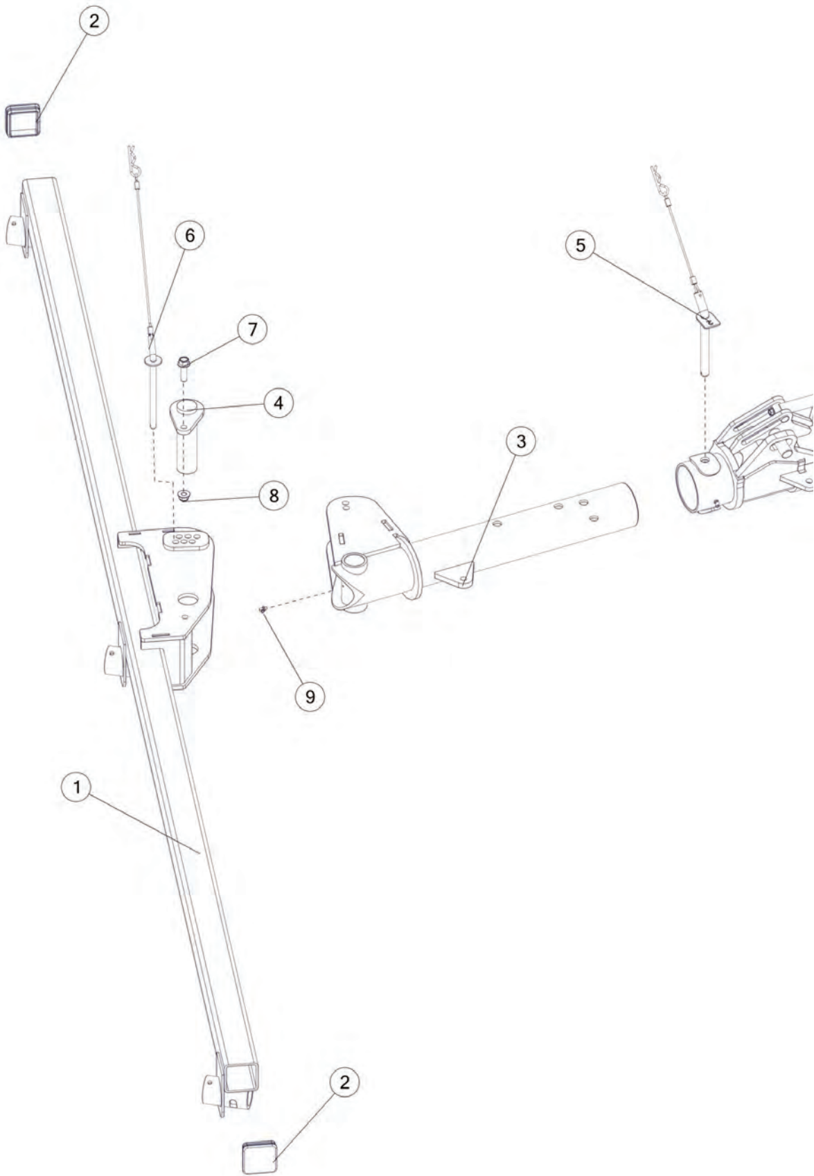
FIGURE 3 LIFT ARM PIVOT & COMPONENTS RH
