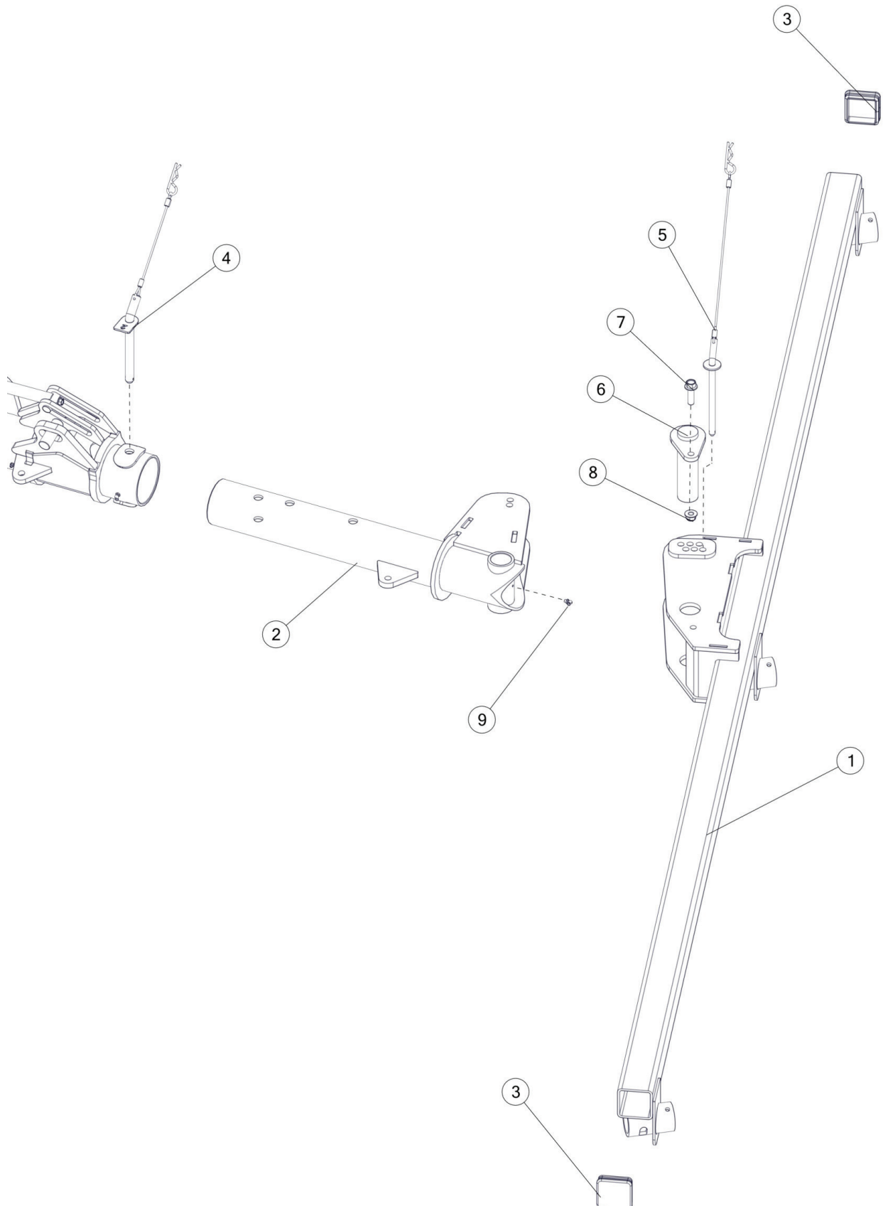
LIFT ARM PIVOT & COMPONENTS LH
