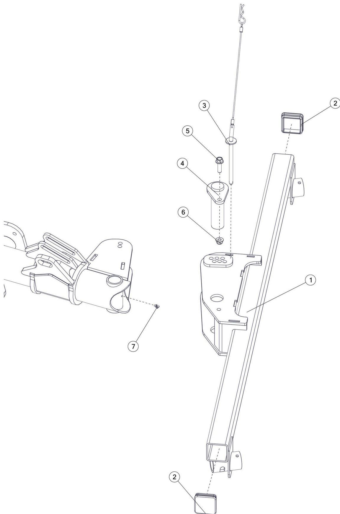
FIGURE 4 LIFT ARM PIVOT & COMPONENTS LH
