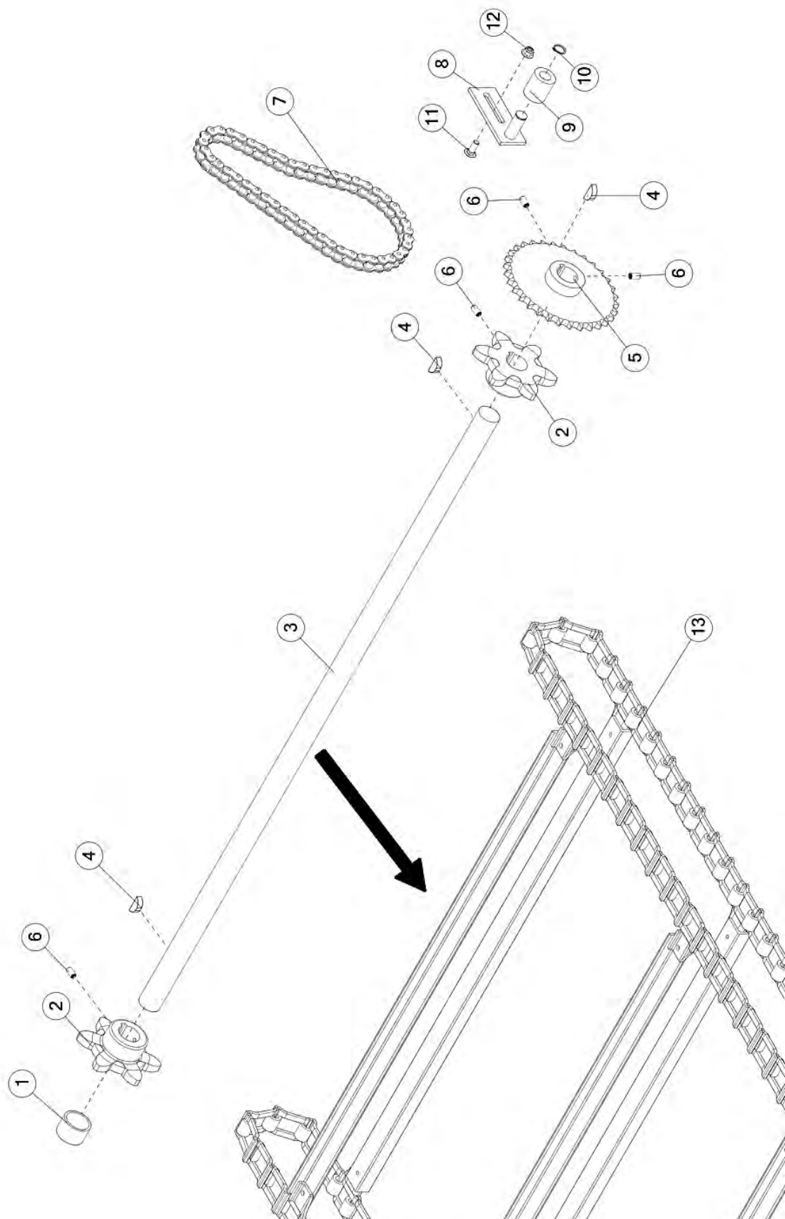
FIGURE 8 APRON CHAIN & REAR DRIVE SHAFT ASSEMBLY
