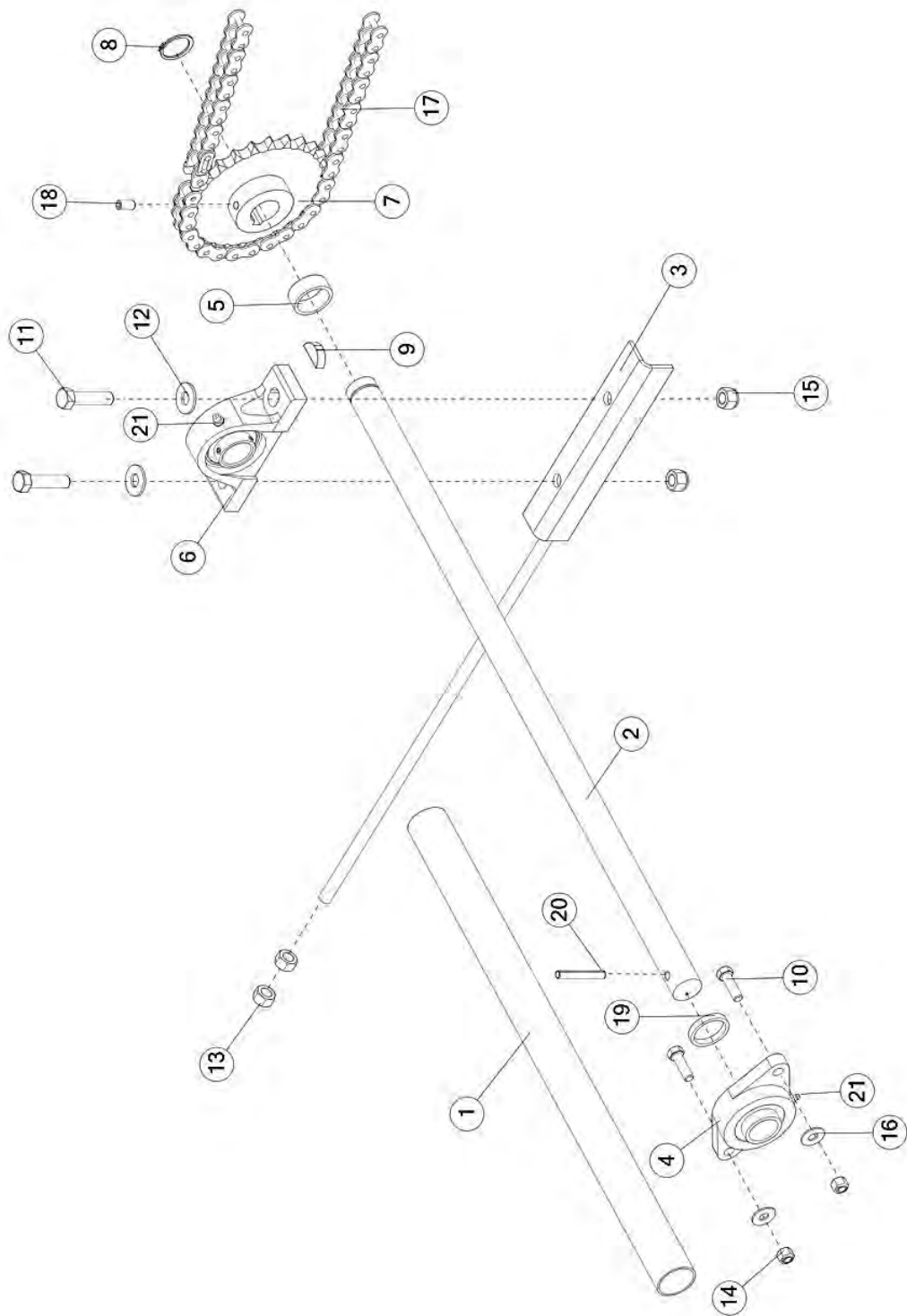
FIGURE 3 FRONT SHAFT ASSEMBLY
