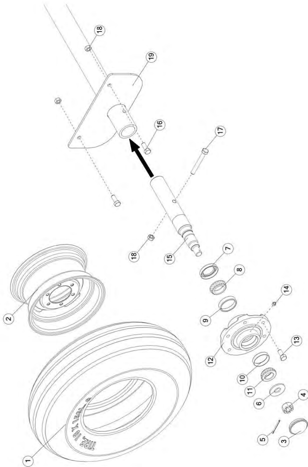
FIGURE 14 HUB ASSEMBLY
