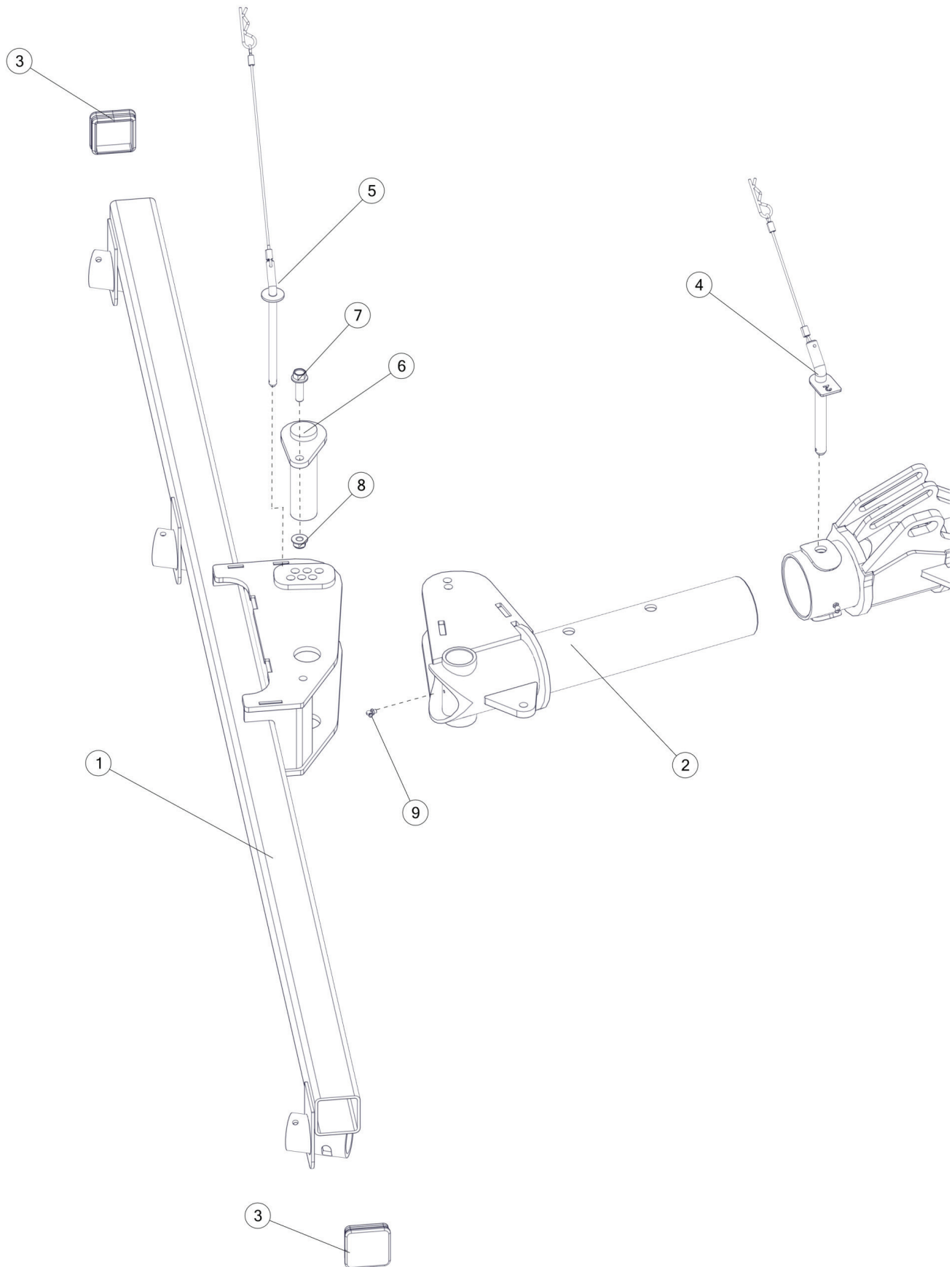
FIGURE 3 LIFT ARM PIVOT & COMPONENTS RH
