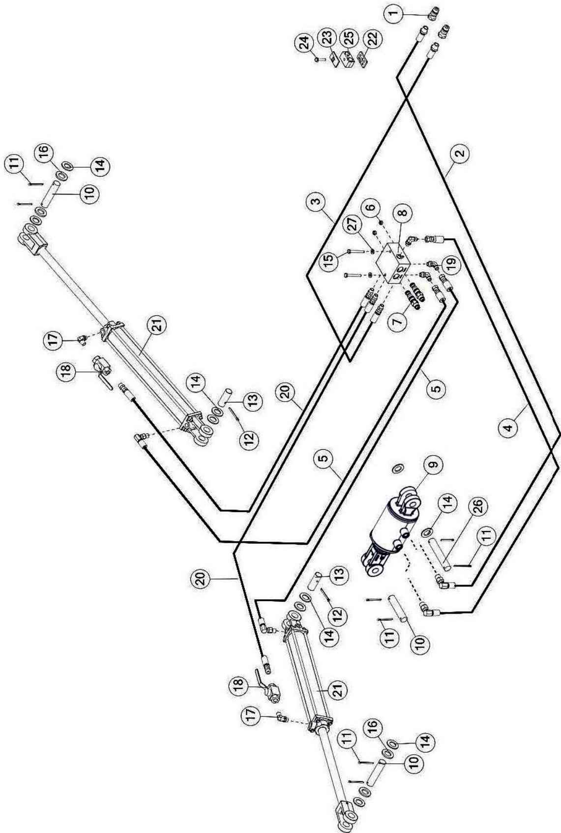
FIGURE 7 HYDRAULICS
