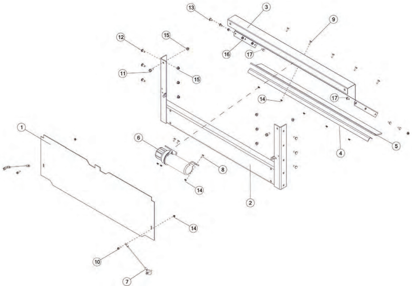
FIGURE 2 FRONT SHIELD & COMPONENTS
