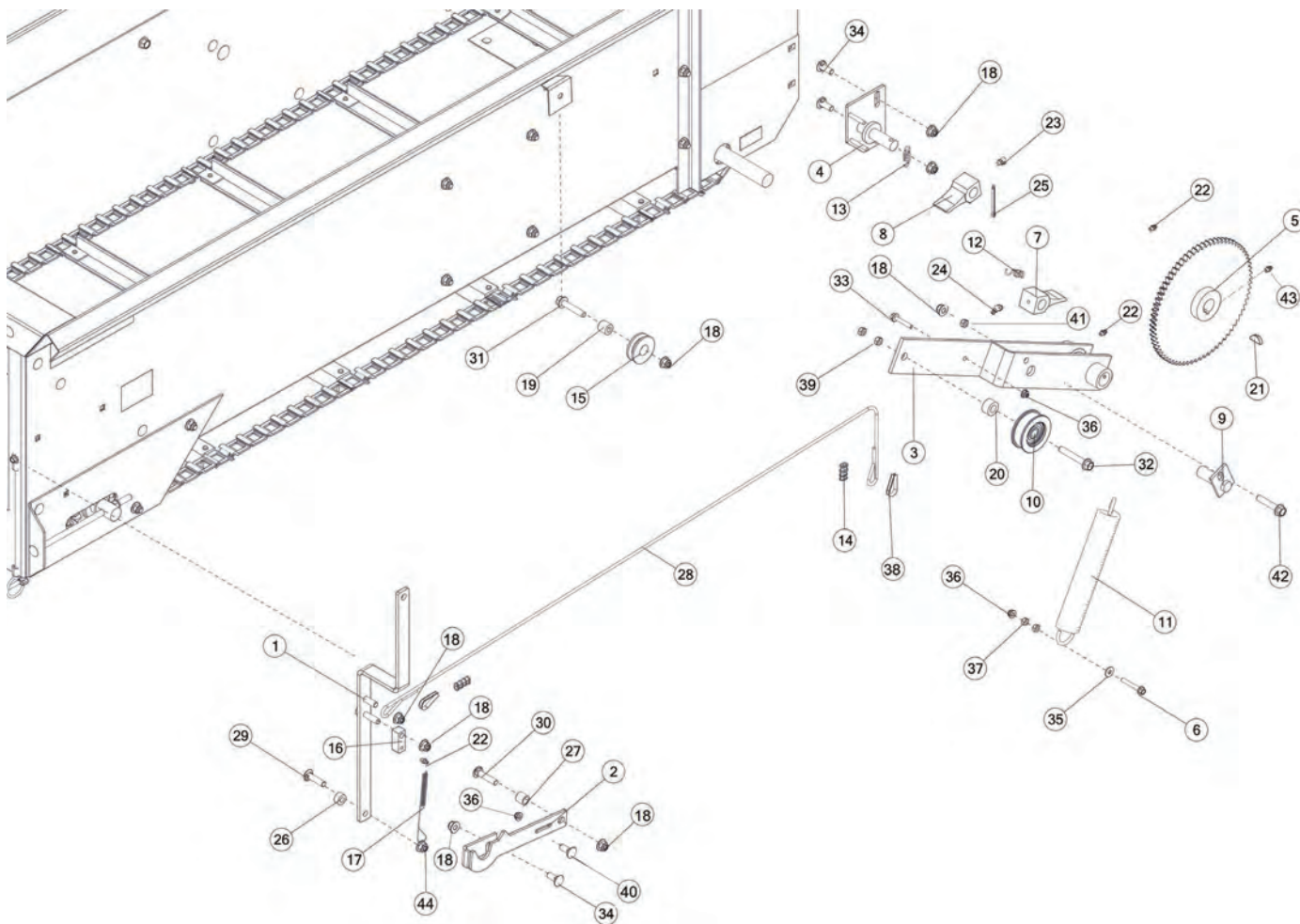
FIGURE 3 DRIVE & COMPONENTS
